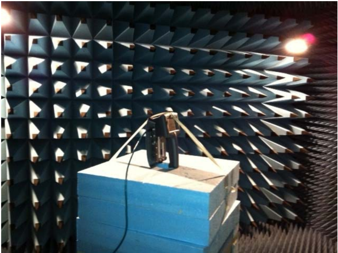
HR-2 - Radiated spurious emission 1-10 GHz
