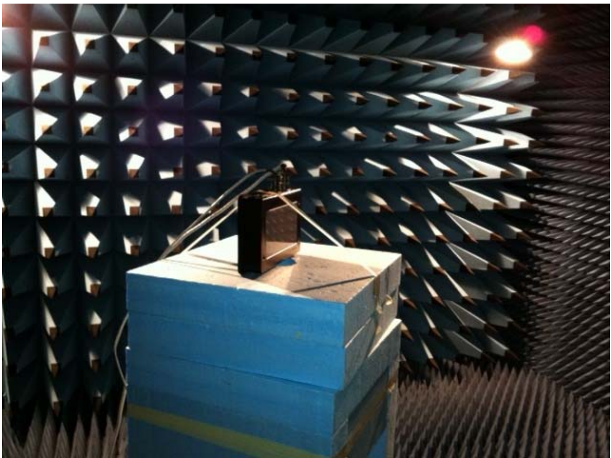
S1566 - Radiated spurious emission 1-10 GHz
