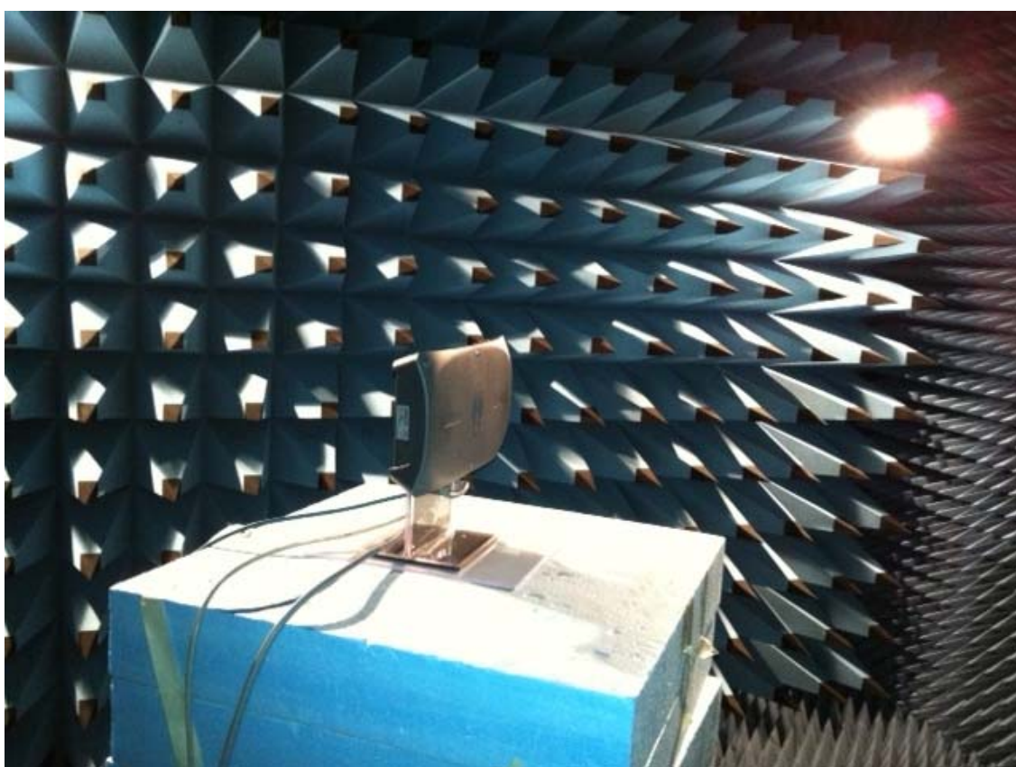
LR-6 - Radiated spurious emission 1-10 GHz
