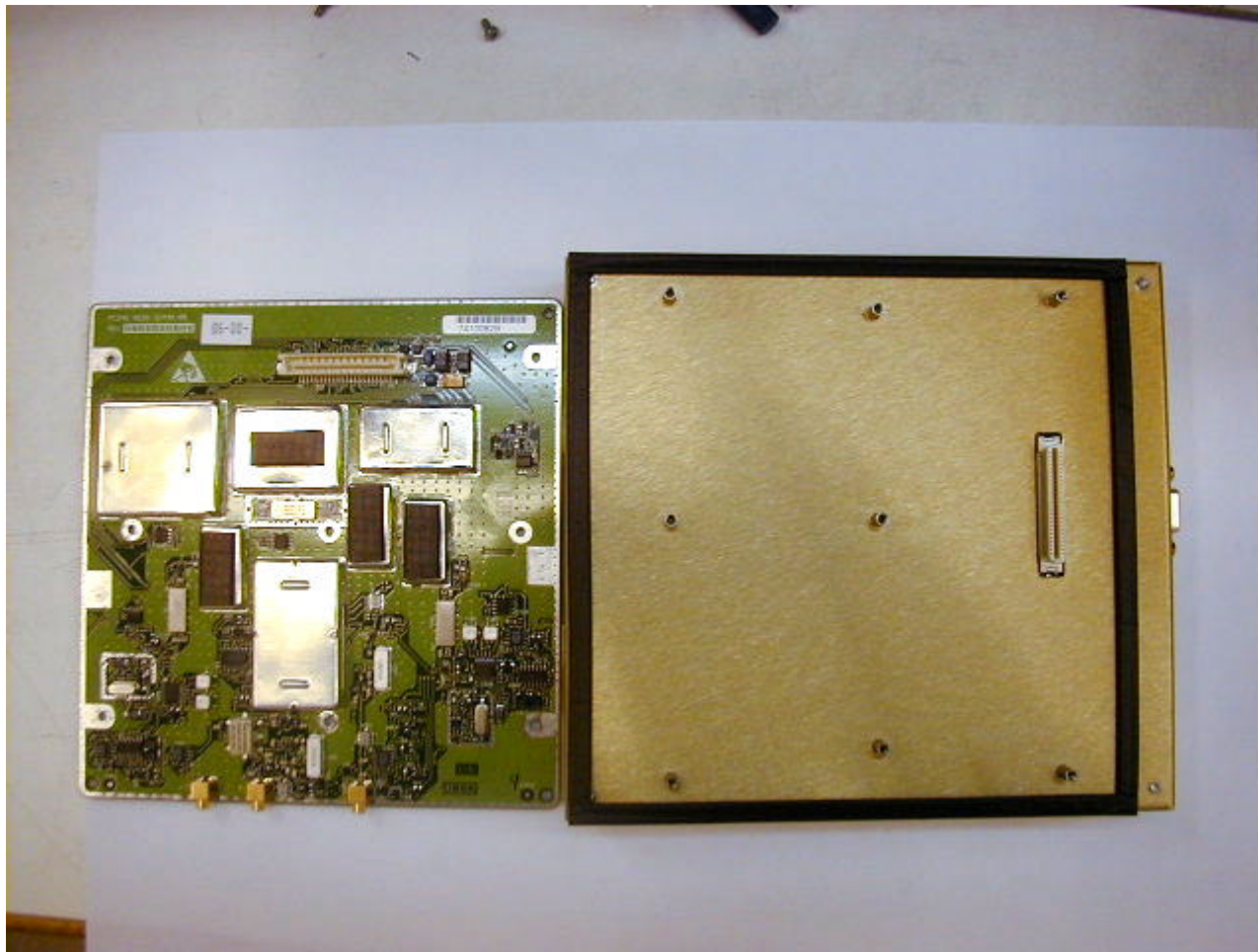
RPC-subassembly bottom view
