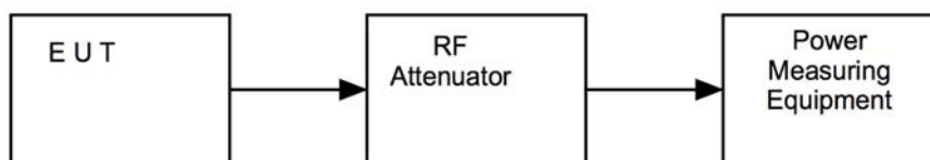
Figure viii Test Setup
