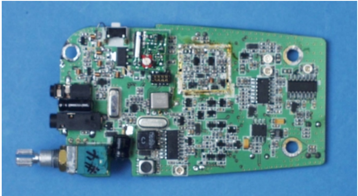
PCB, Without Shields
