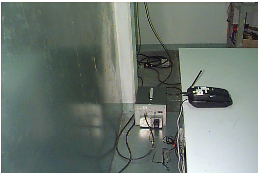
Conducted Emissions Test Set-up Rear View
