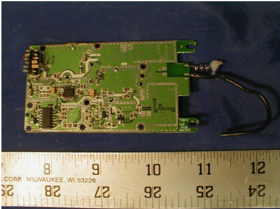
Component view
