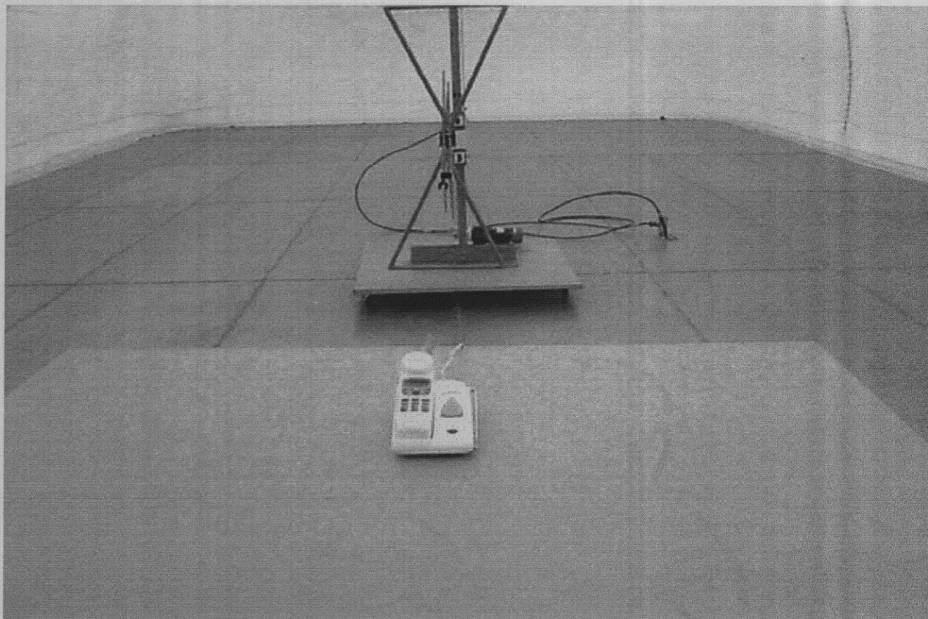
Radiated Emission Test Set-up - Rear View
