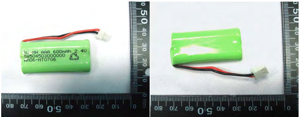
Figure 3. Battery (Ni-MH 2.4V , 600mAh)
