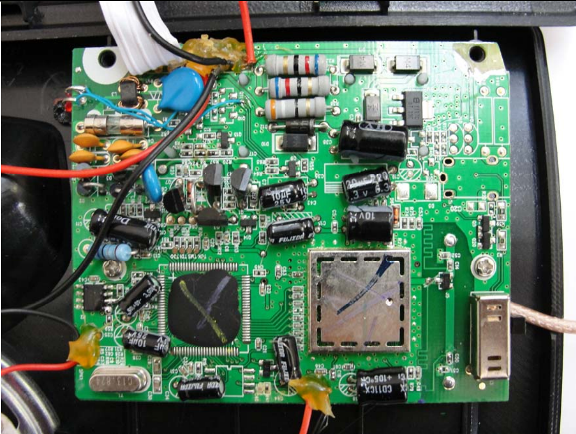
Figure 2: Inside Base
