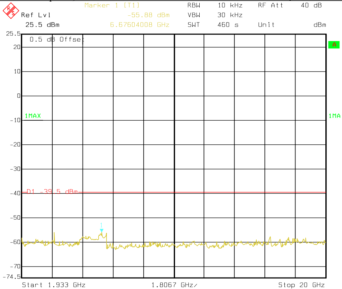
Figure 23: Outside the sub-band High Channel
