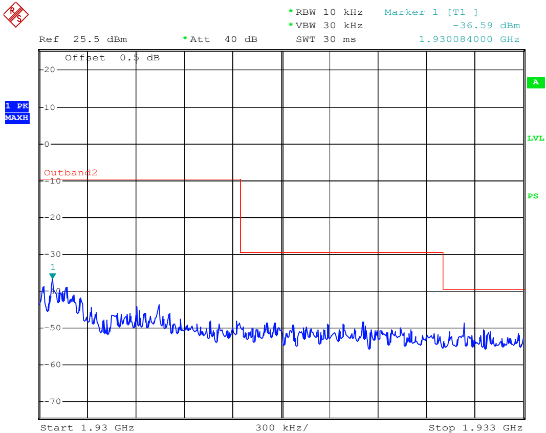
Figure 22: Outside the sub-band High Channel
