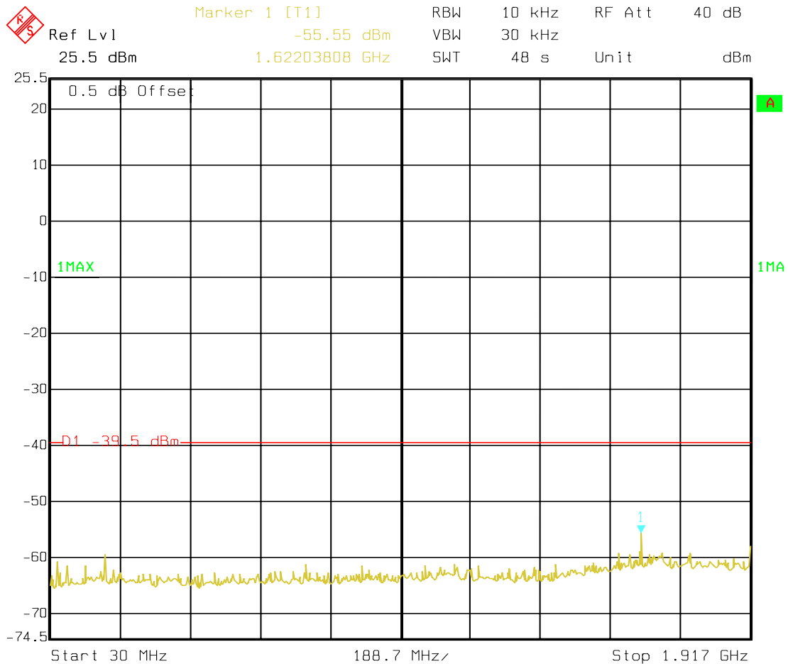
Figure 16: Outside the sub-band Low Channel
