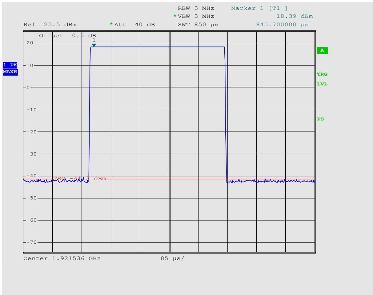
Figure 2: MID channel Peak transmit power
