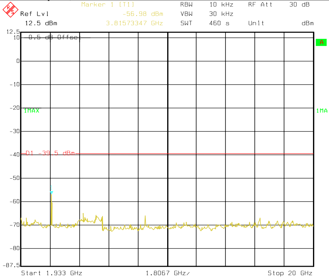
Figure 19: Outside the sub-band Low Channel
