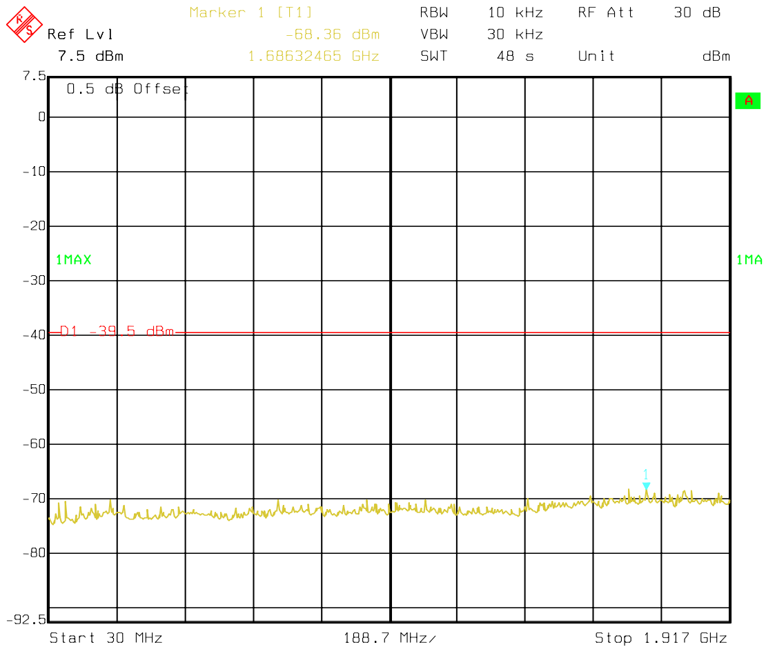
Figure 20: Outside the sub-band HIGH Channel
