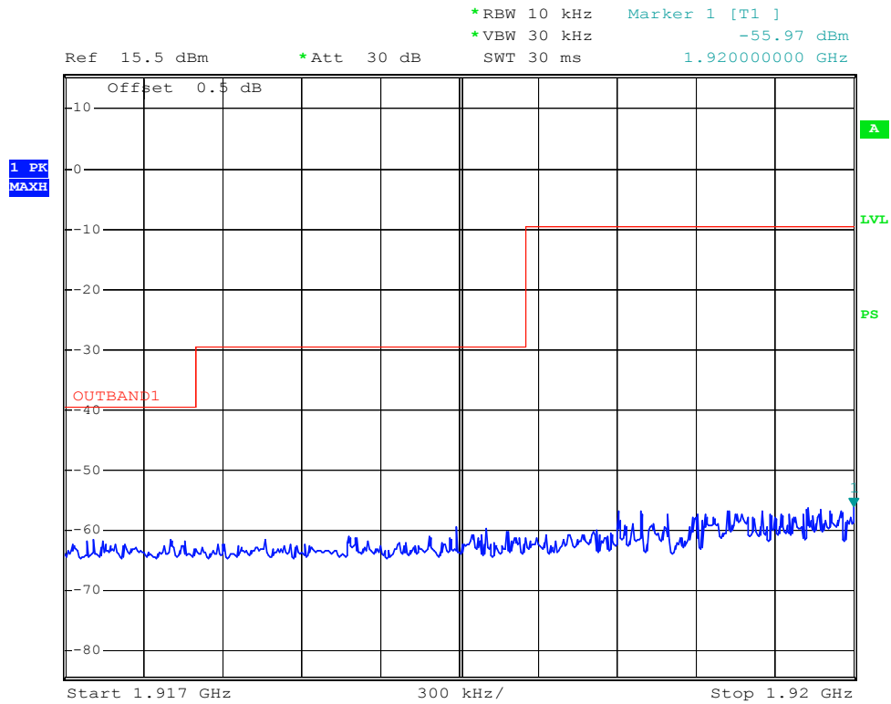
Figure 21 Outside the sub-band High Channel
