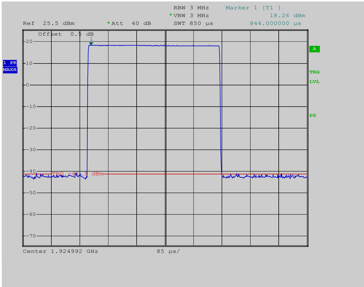
Figure 3: First channel Peak transmit power
