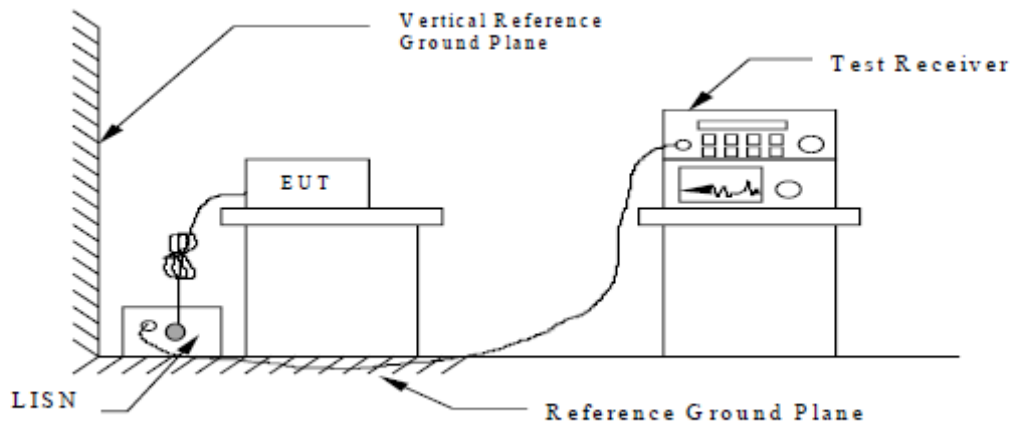
Test Set-up 4
