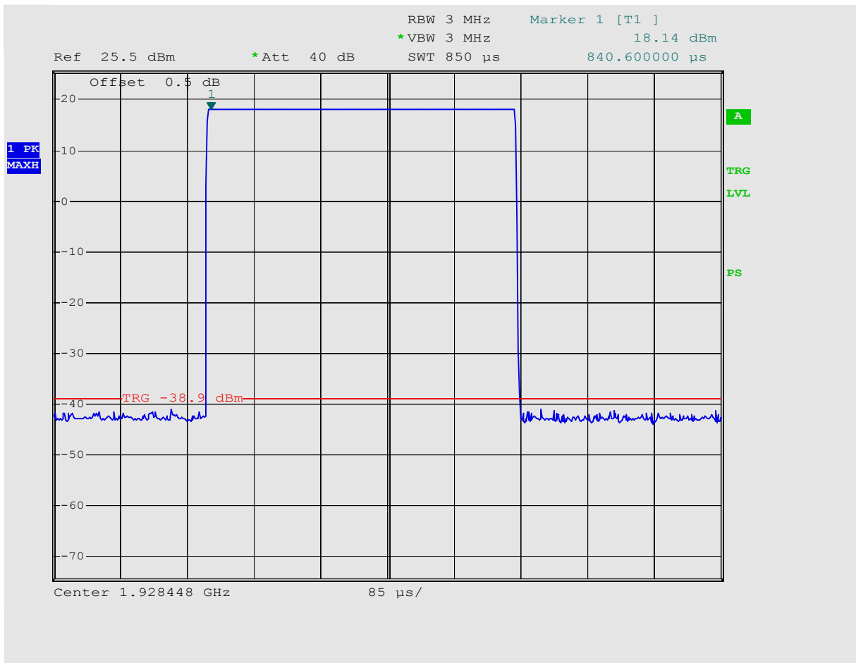
Figure 1: Last channel Peak transmit power
