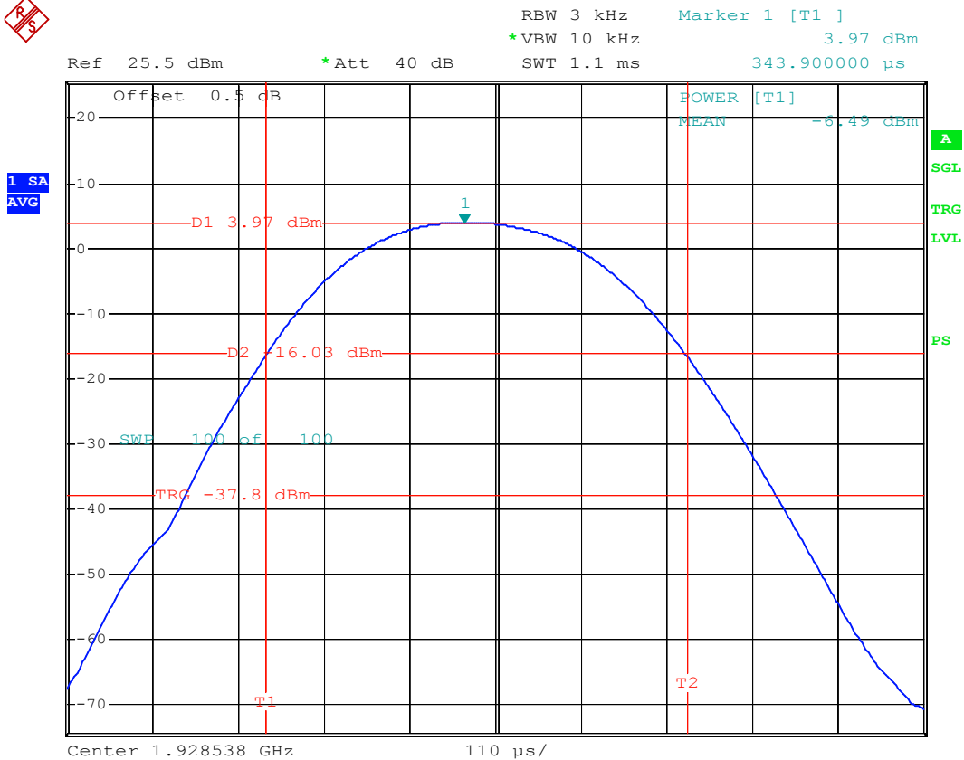
Figure 9: Last channel power spectral density
