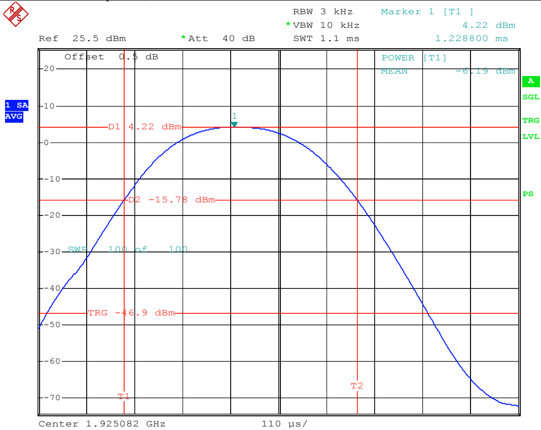
Figure 7: MID channel power spectral density
