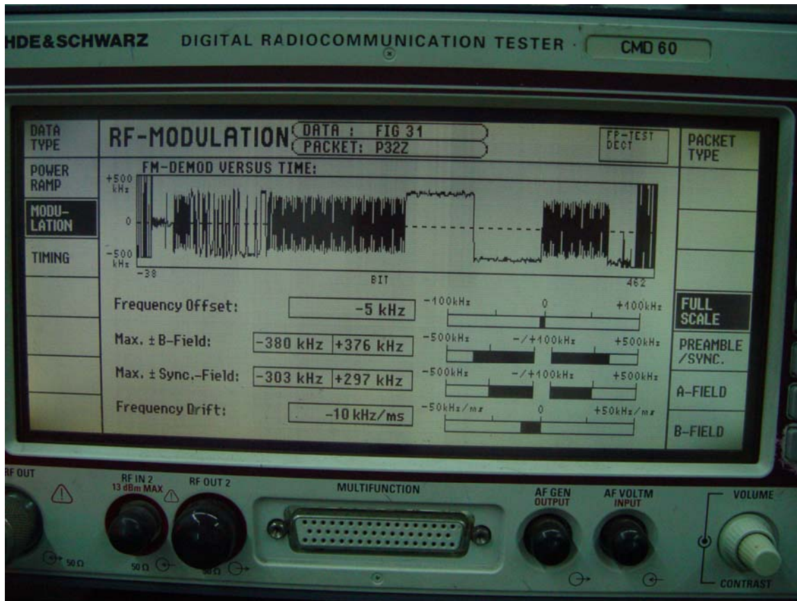
Figure 24: Frequency Stability
