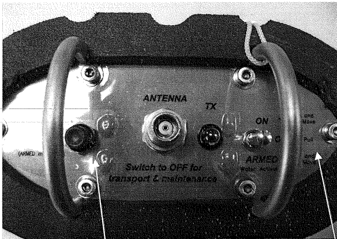
Part number & FAA label location on ELT model ADT 406 S
