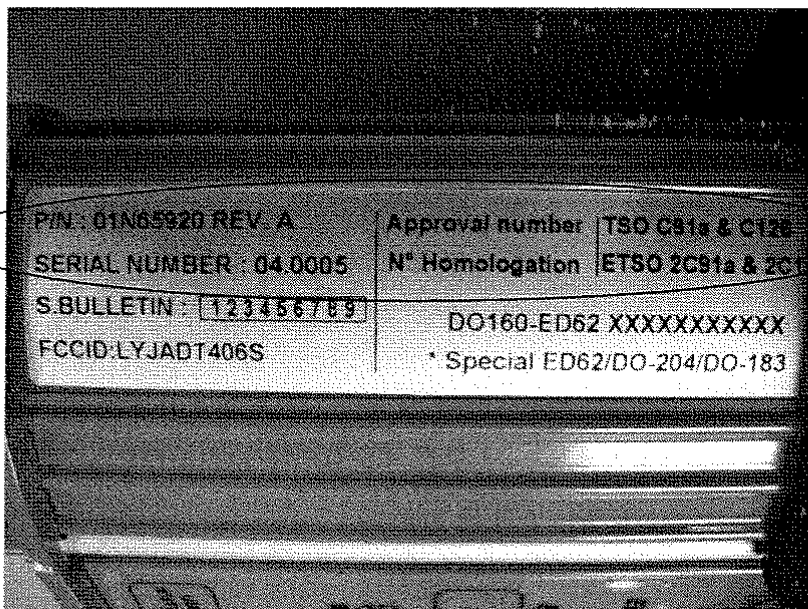
Part number & FAA label location on ELT model ADT 406 S
