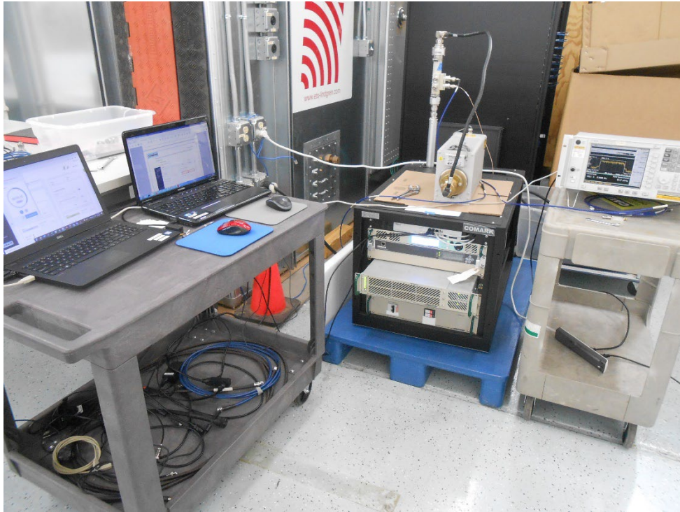
Conducted RF
