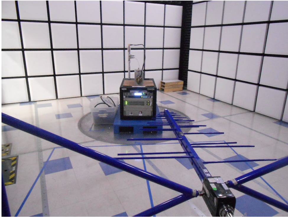
Radiated RF below 1 GHz
