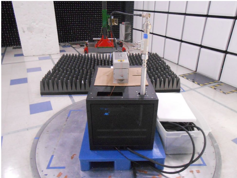
Radiated RF above 1 GHz
