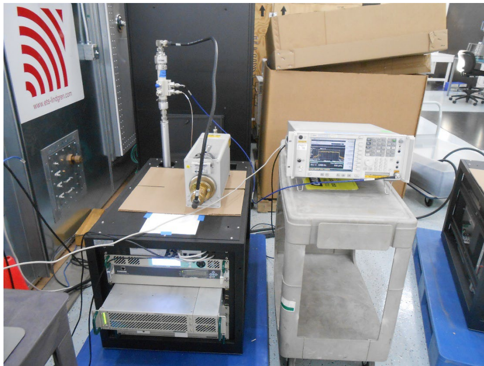
Conducted RF at PA output
