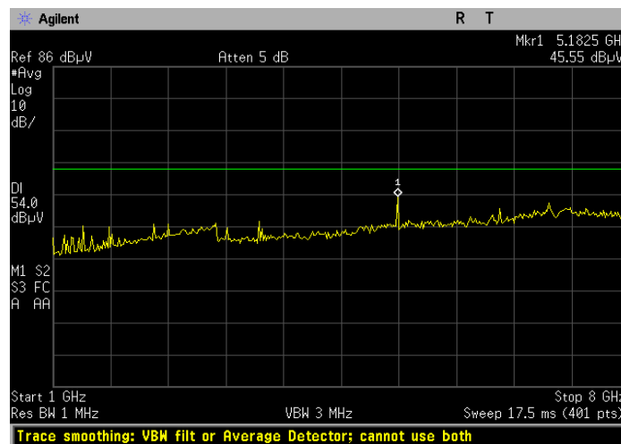
Figure 5-15 Test Plot for Horizontal Radiated Emissions Above 1 GHz
