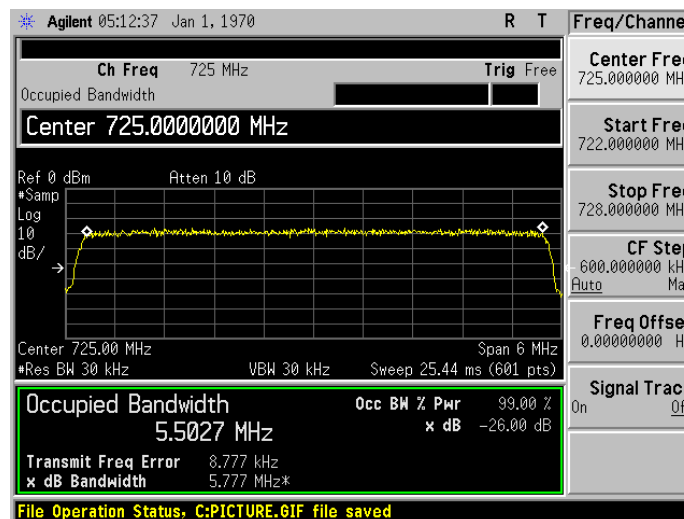
Figure 5-4 Occupied Bandwidth Plot
