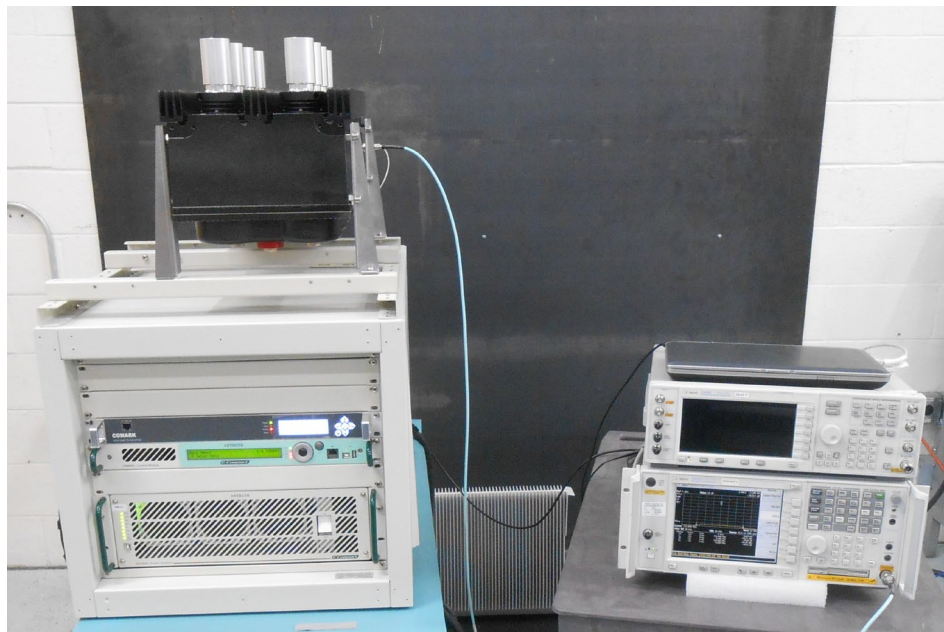
Figure 5-2 Photo of Power Measurement Test Set-Up
