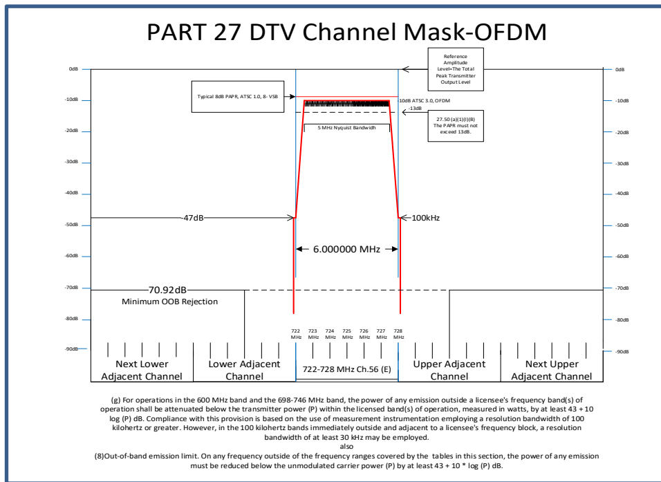
Figure 5-8 FCC Part 27 Spectral Mask
