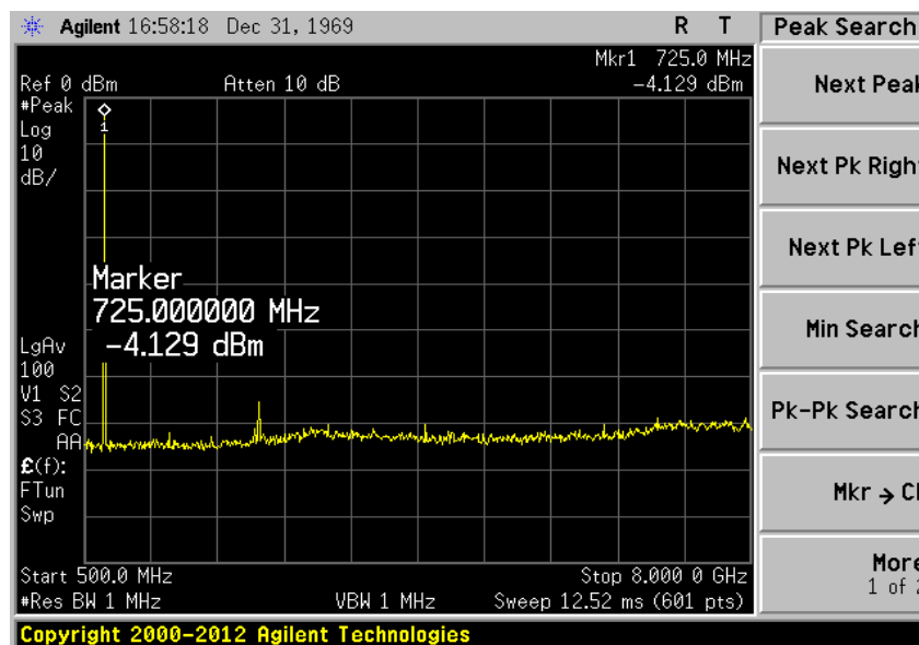
Figure 5-9 Harmonic Emissions at Antenna Terminals
