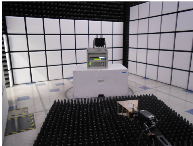
Figure 5-14 Test Set-Up for Radiated Emissions Above 1 GHz
