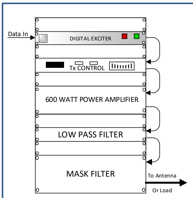
Figure 4-1 System Signal Flow Diagram
