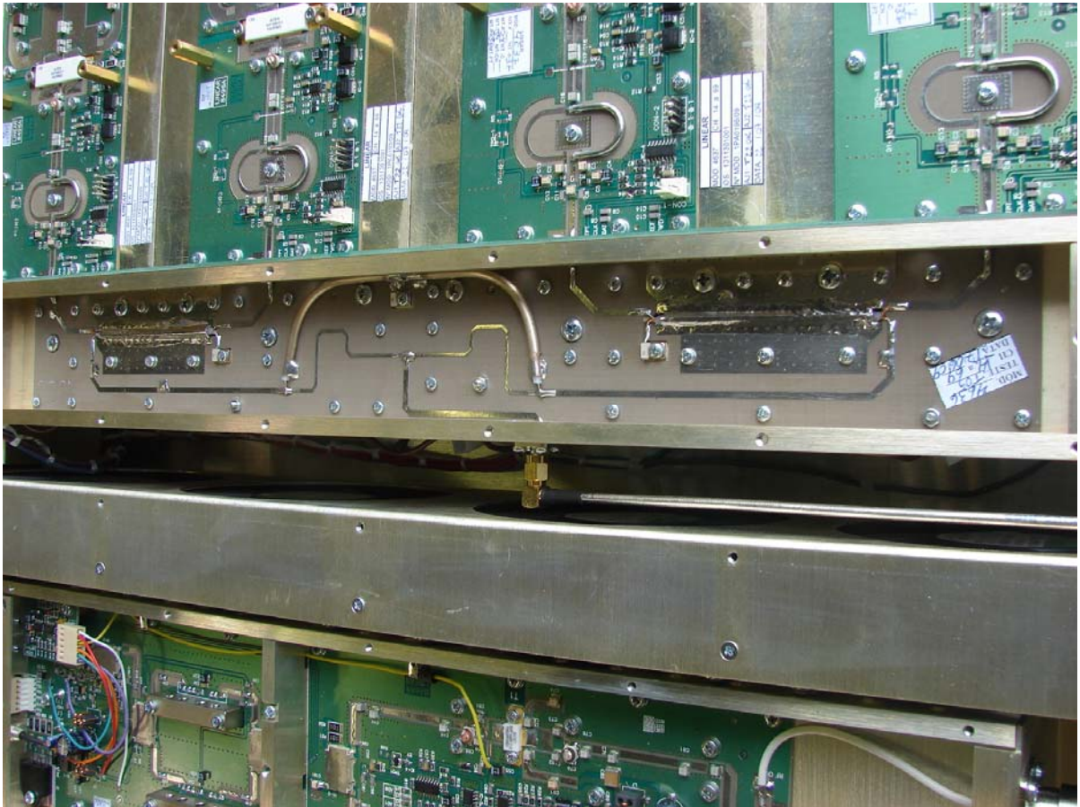
1:4 Splitter
