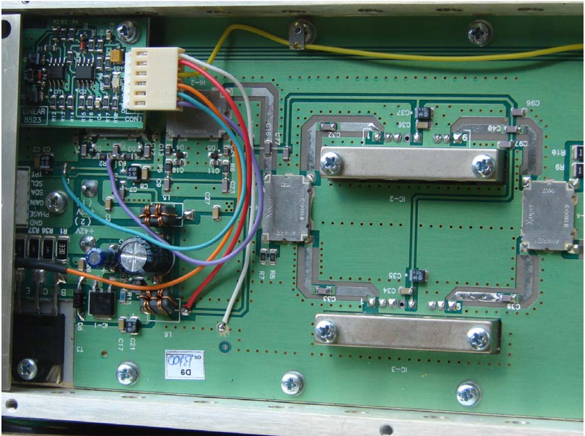
Stage 1 and Stage 2 Driver
