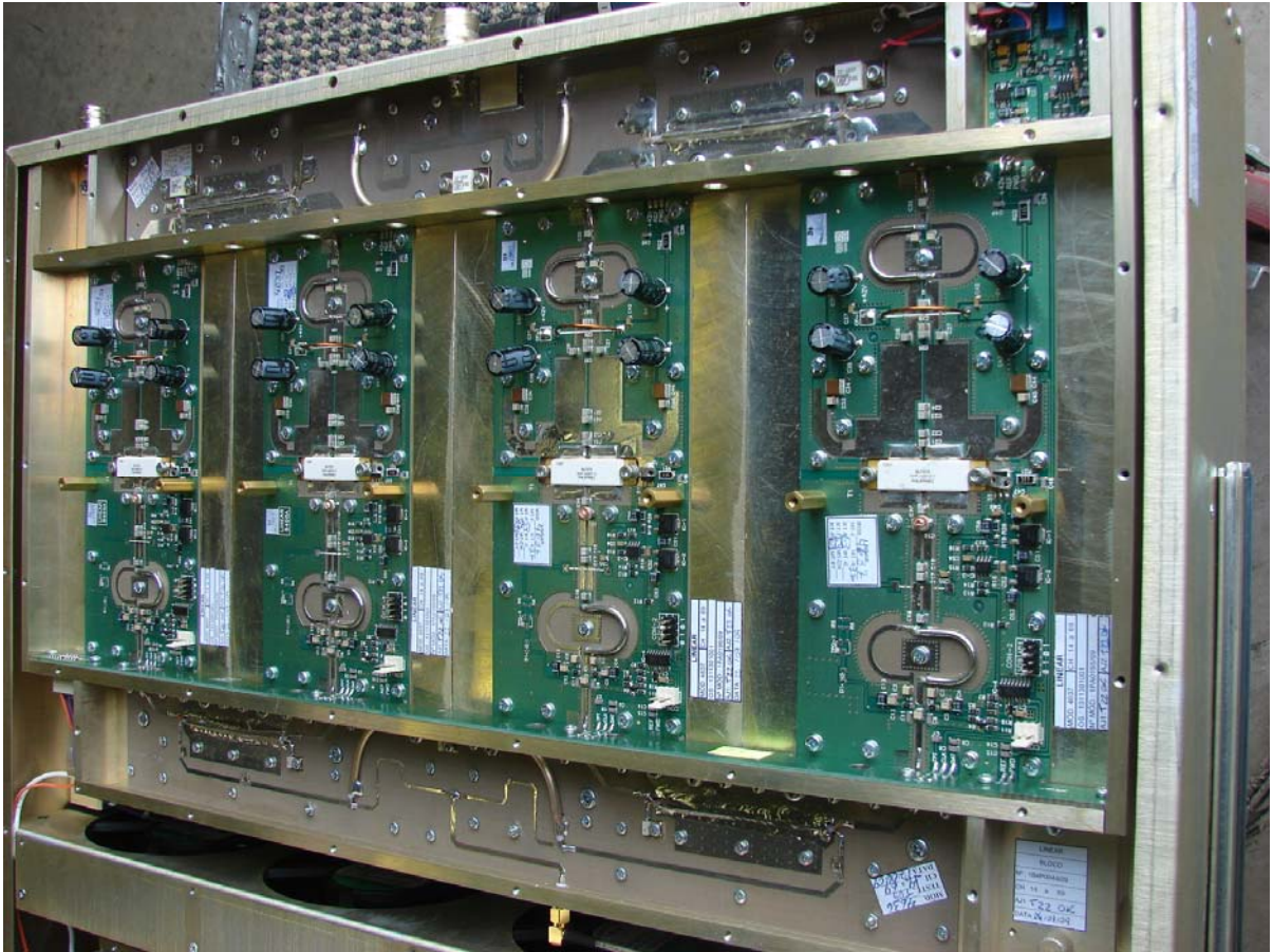
4 x 107w Pallet Amplifiers Setup + Splitter + Combiner
