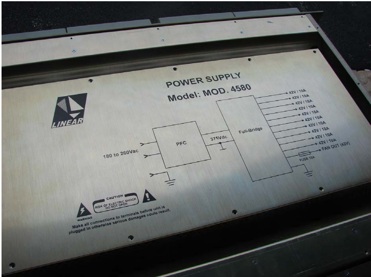
Power Supply
