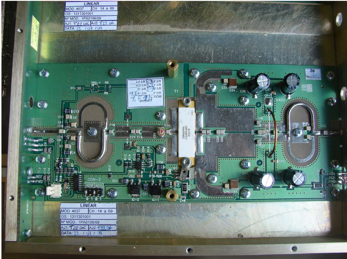
107W Pallet Ouput RF Amplifier
