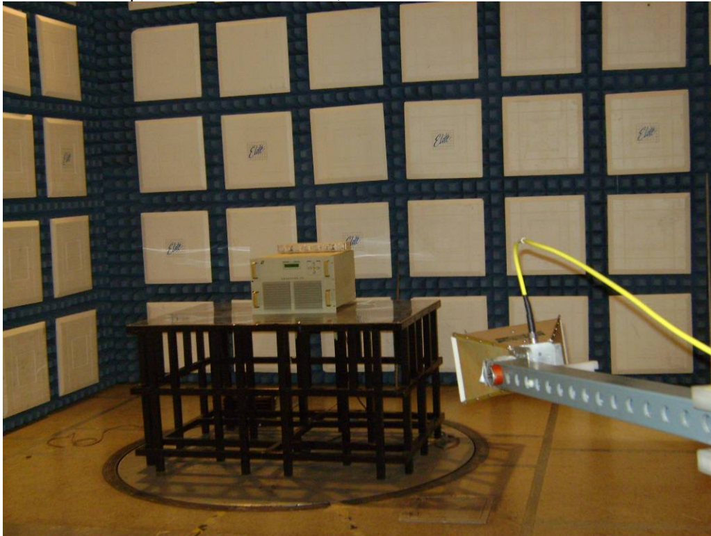
Test Set-up for Radiated Emissions, 30MHz to 5GHz – Vertical Polarization
