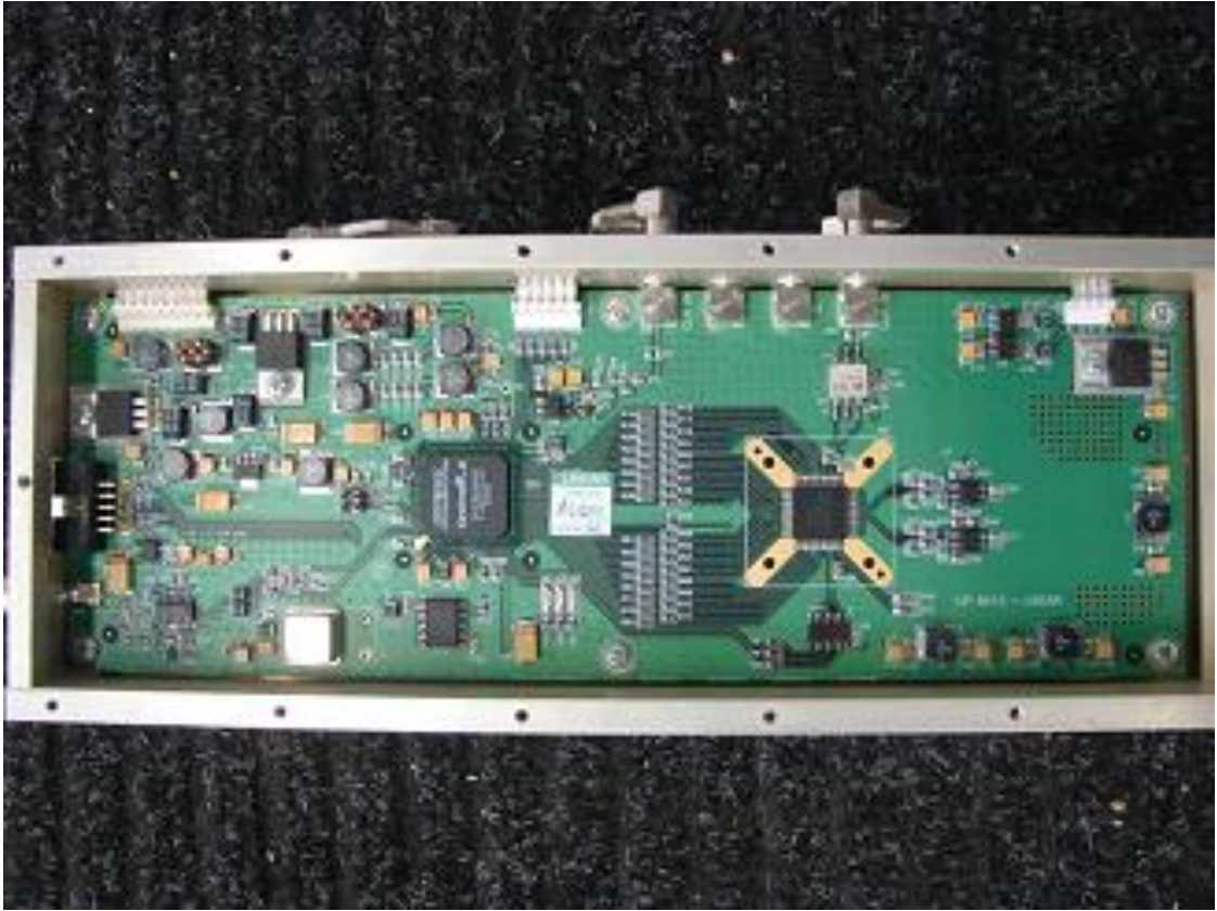
AT7120 ATSC Modulator
