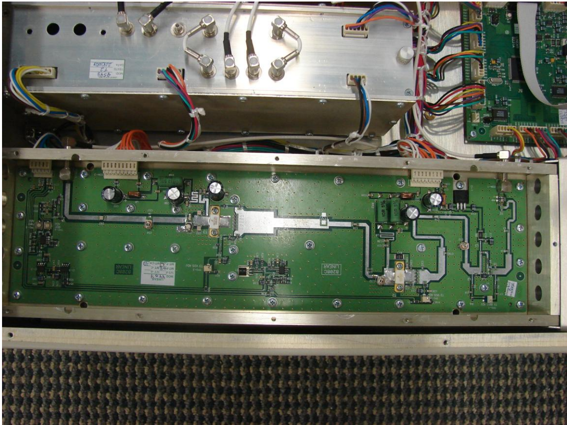
AT7120 – Driver Amplifier
