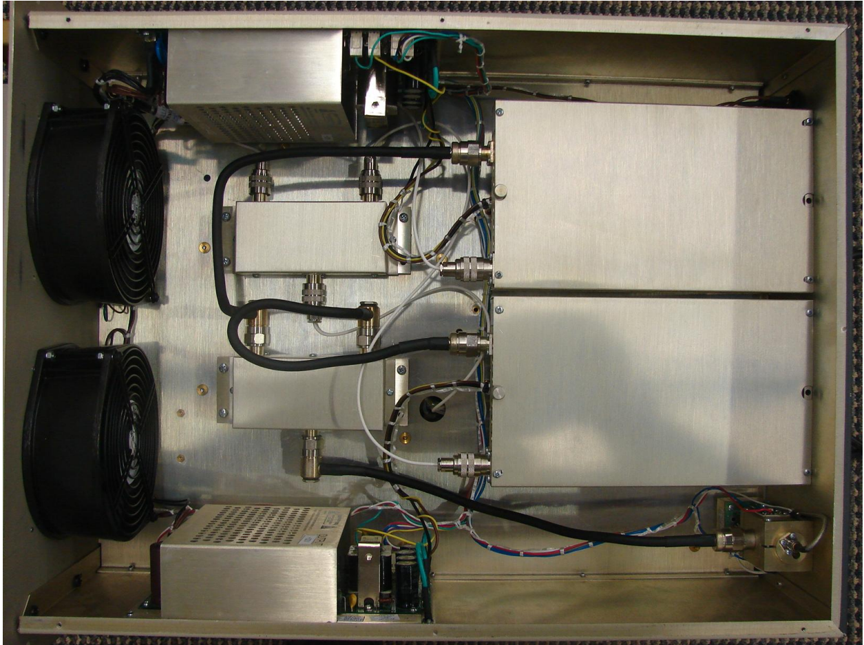
AT7120 Bottom View
