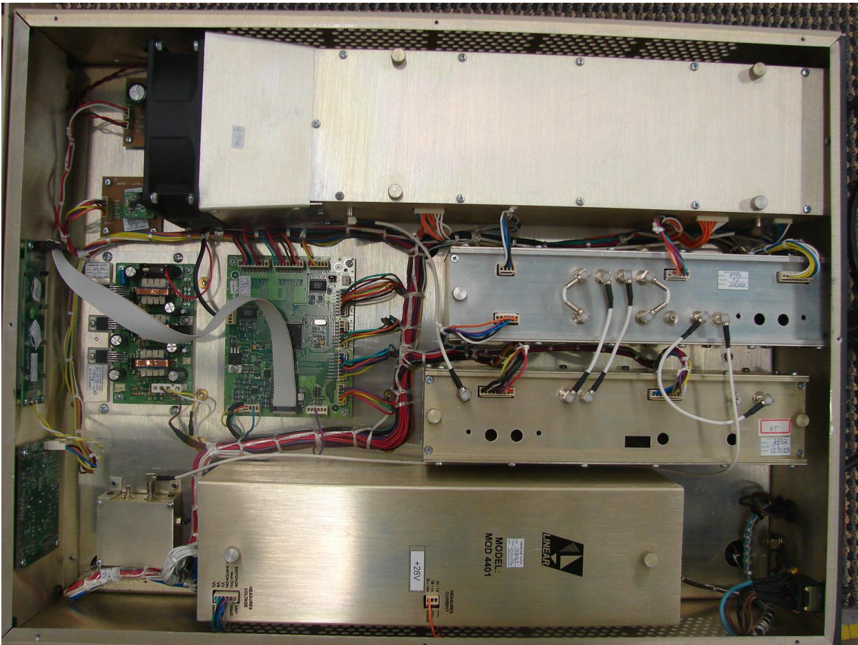
AT7120 Top View of the Unit
