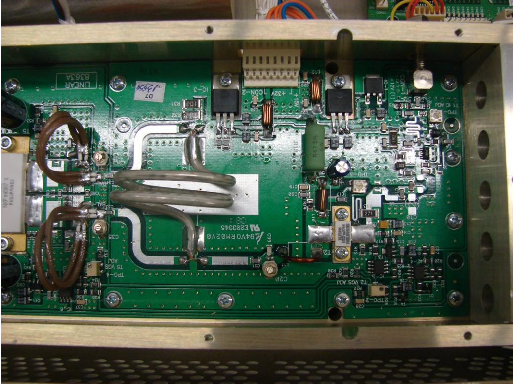
50W Multistage VHF Amplifier – RF Transistor Input Circuit Matching
