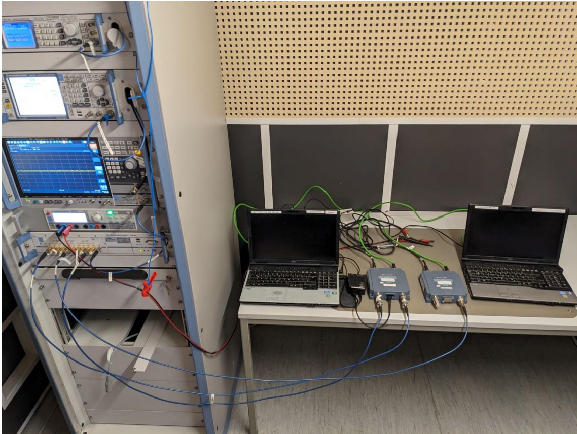
Photo 1: Test setup for conducted DFS tests
