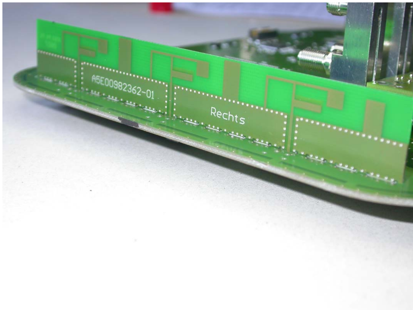
Antenna A5E00982362
