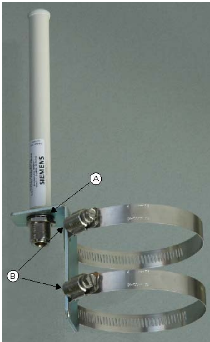
Figure 0-1 Option for Mounting the ANT793-6MN on a Mast
