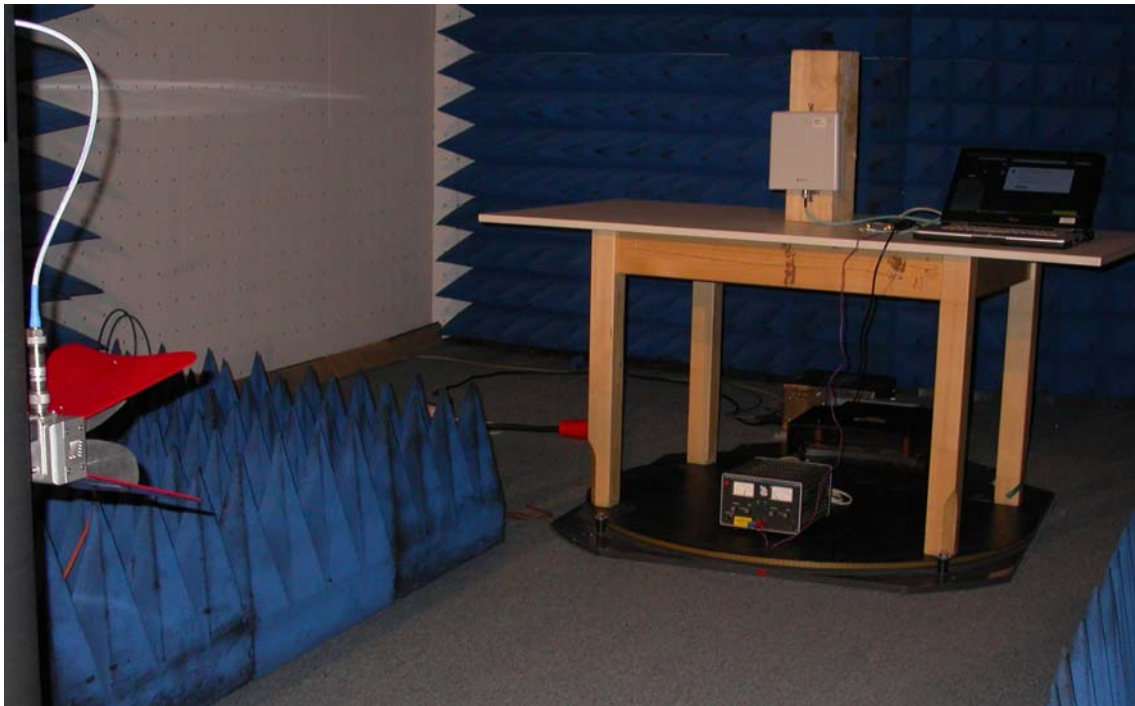
Anechoic chamber
