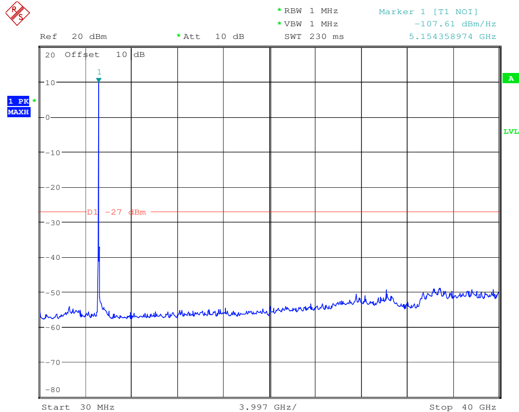
Plot 1: 5180 MHz
