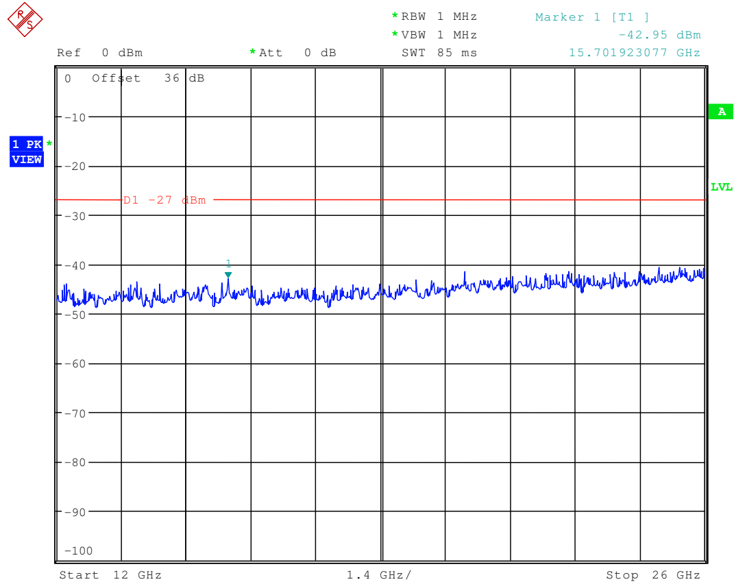
Plot 4: 12 GHz - 26 GHz vertical (valid for all channels)
