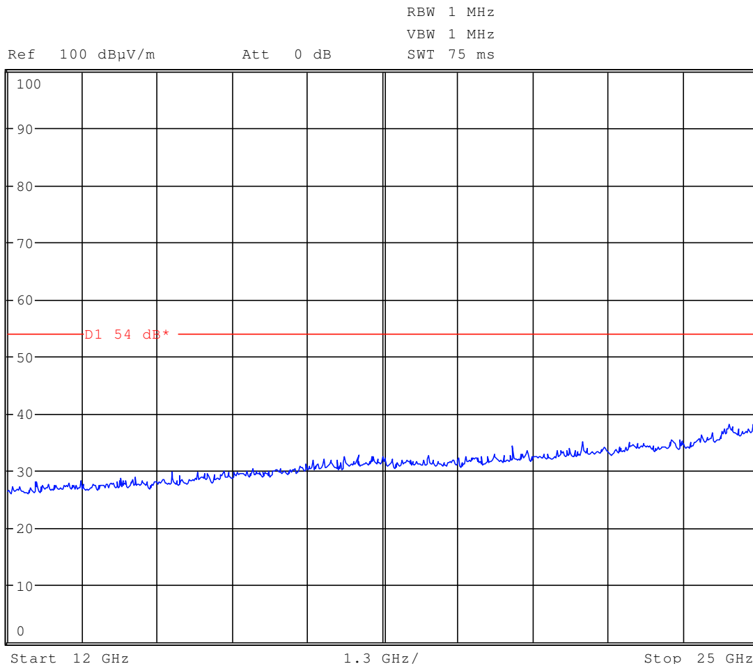
Plot 3: - 25 GHz
