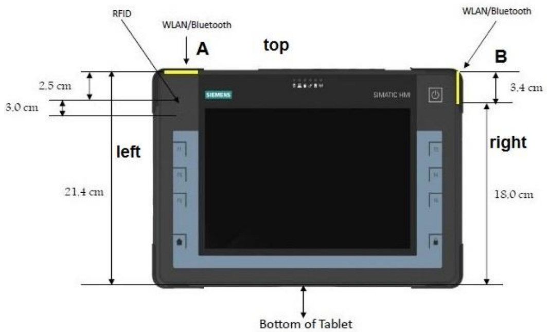
Photo 12: Antennae position
