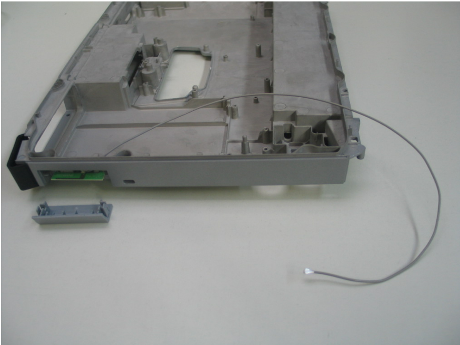
Photo 8: external antenna (in TFT housing)
