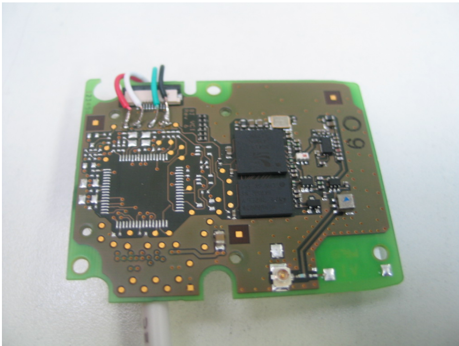
Photo 6: EUT (top side)
