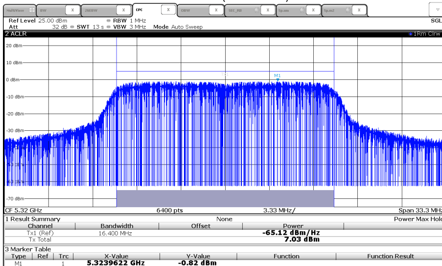
Channel 64 (5320 MHz)
