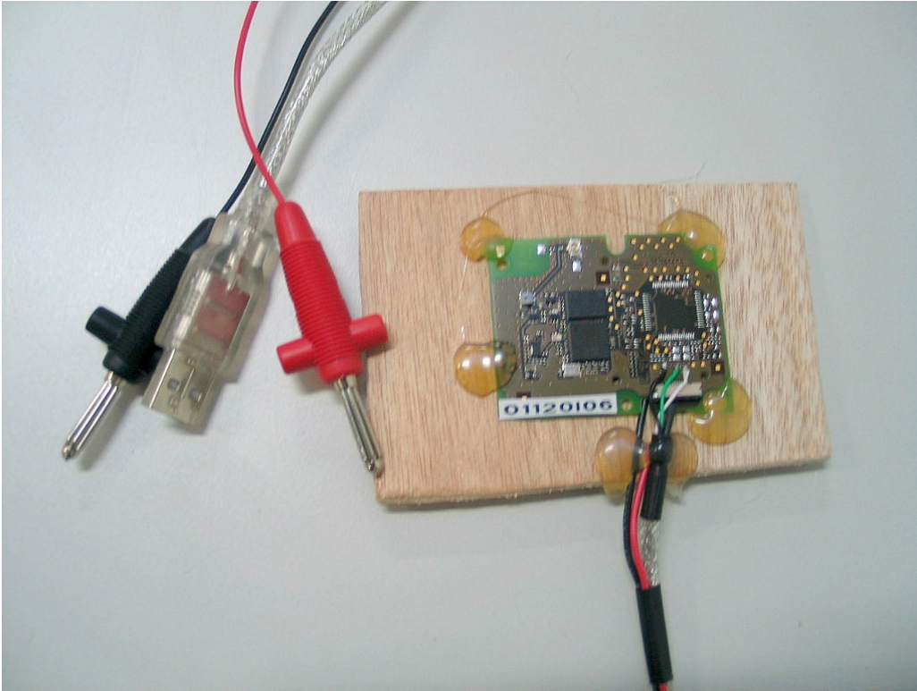
Photo 5: EUT (mounted on a piece of wood – only to improve the mechanical stability during the tests)
