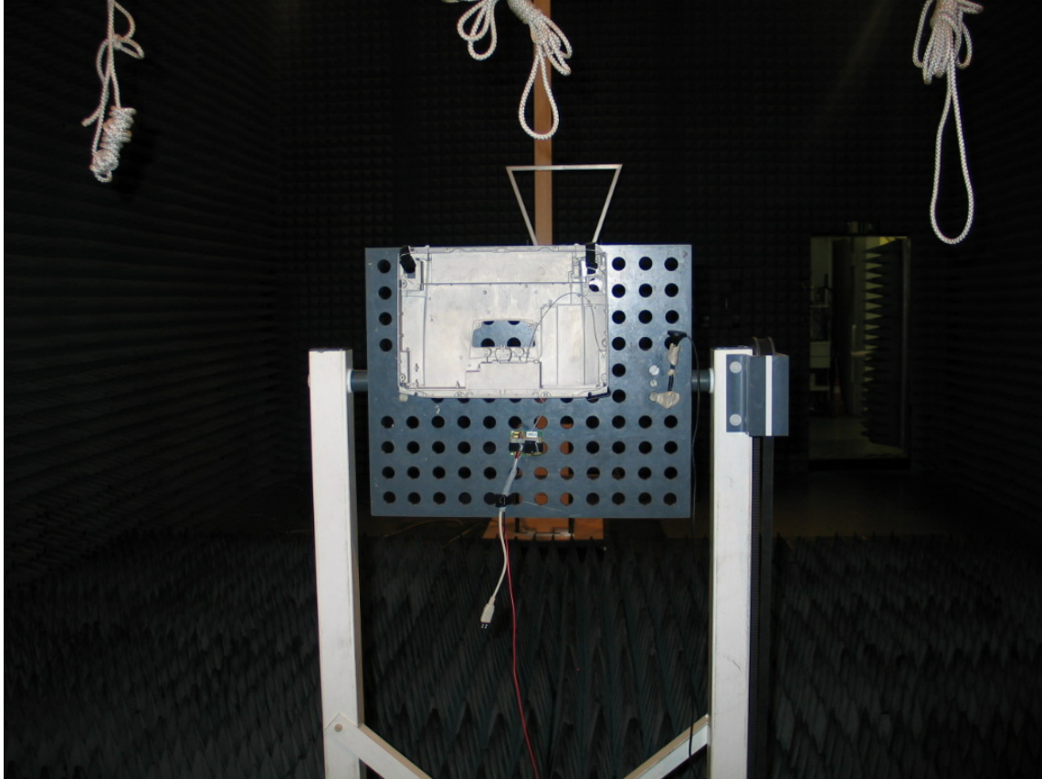
Photo 1: Test setup for radiated measurements (module + external antenna, above 1 GHz)
