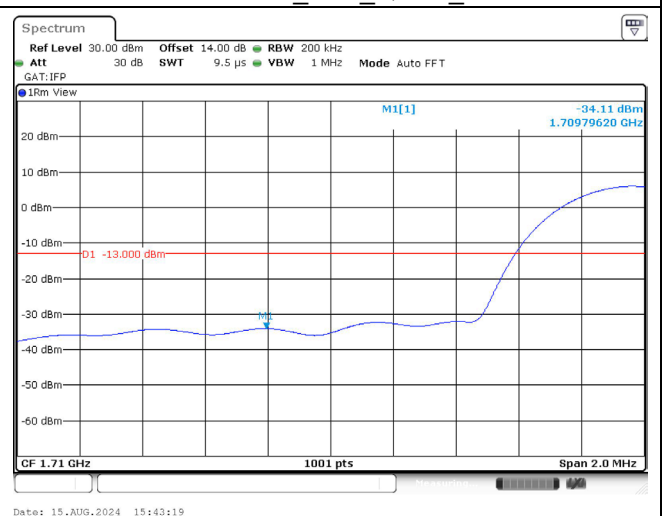
1717.5 MHz_15M_QPSK_FRB
