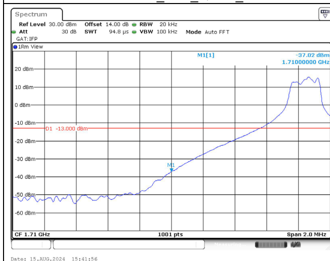
1717.5 MHz_15M_QPSK_1RB
