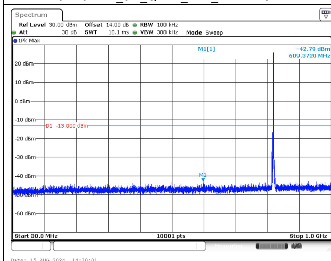
822.5 MHz_3M_QPSK_1RB_Below 1GHz
