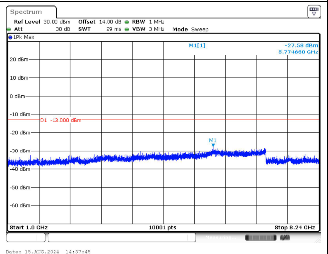
819.0 MHz_5M_QPSK_1RB_Above 1GHz
