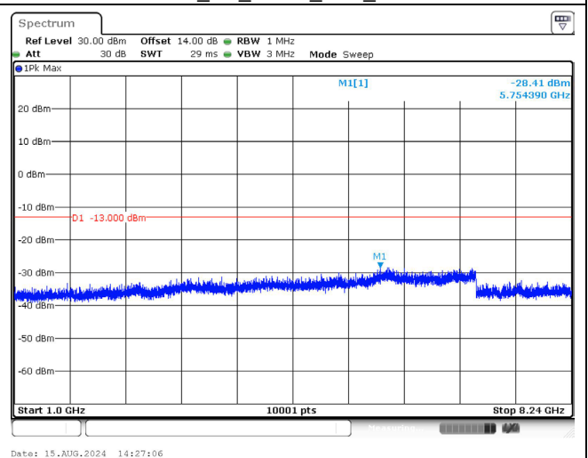
822.5 MHz_3M_QPSK_1RB_Above 1GHz
