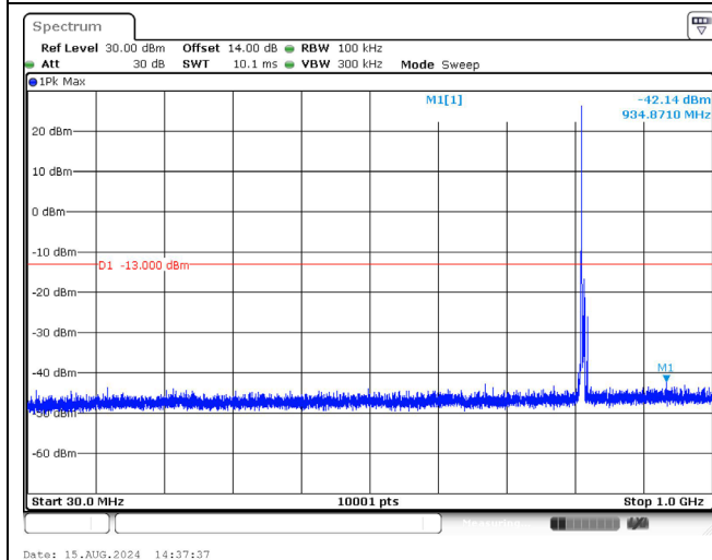
819.0 MHz_5M_QPSK_1RB_Below 1GHz
