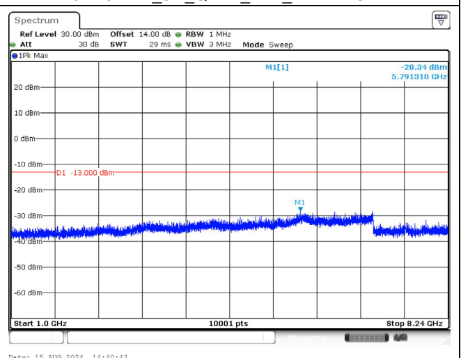
821.5 MHz_5M_QPSK_1RB_Above 1GHz
