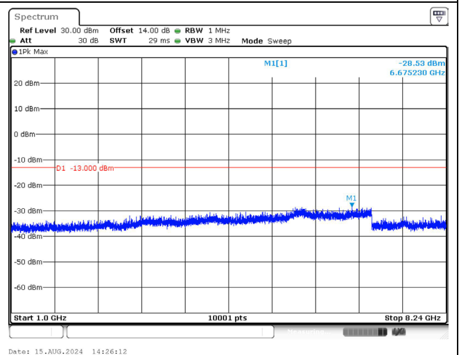
819.0 MHz_3M_QPSK_1RB_Above 1GHz
