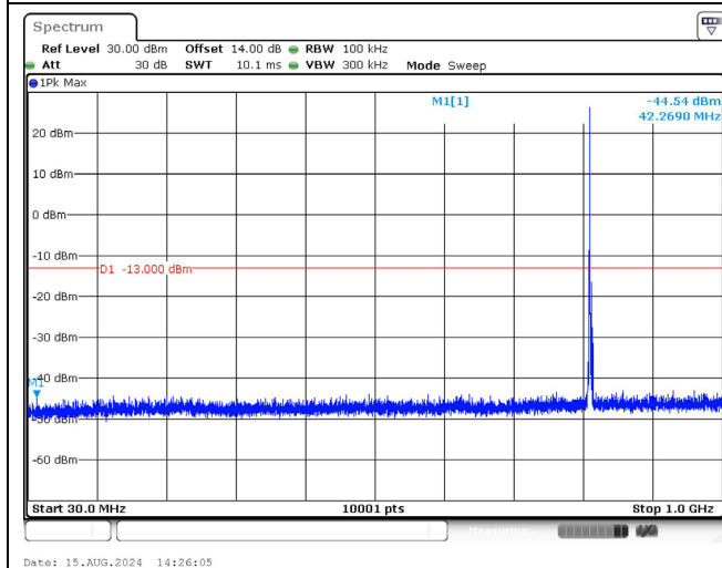
819.0 MHz_3M_QPSK_1RB_Below 1GHz
