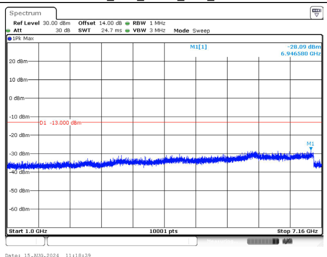
711.0 MHz_10M_QPSK_1RB_Above 1GHz
