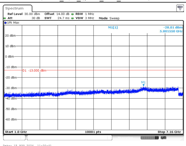
711.0 MHz_10M_QPSK_1RB_Above 1GHz
