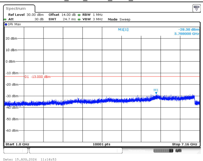
707.5 MHz_10M_QPSK_1RB_Above 1GHz
