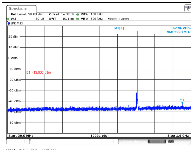
714.5 MHz_3M_QPSK_1RB_Below 1GHz
