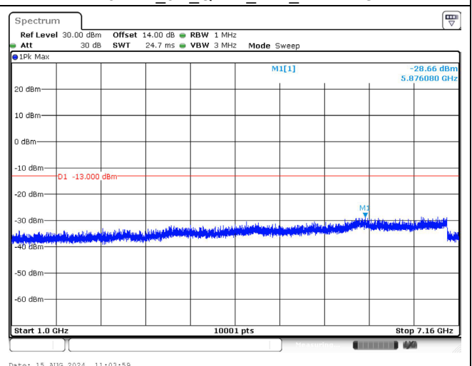
714.5 MHz_3M_QPSK_1RB_Above 1GHz
