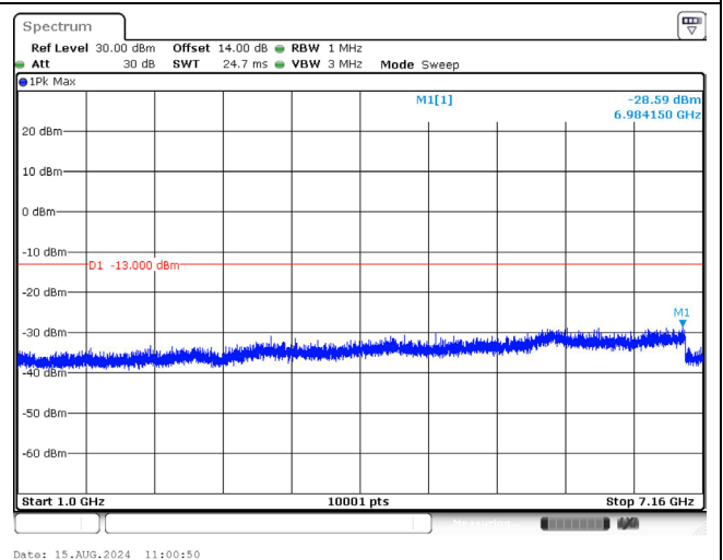
707.5 MHz_3M_QPSK_1RB_Above 1GHz
