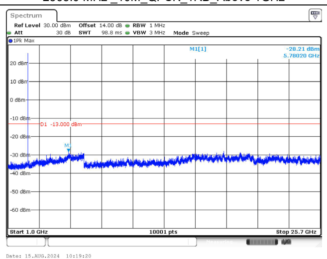
2565.0 MHz_10M_QPSK_1RB_Above 1GHz
