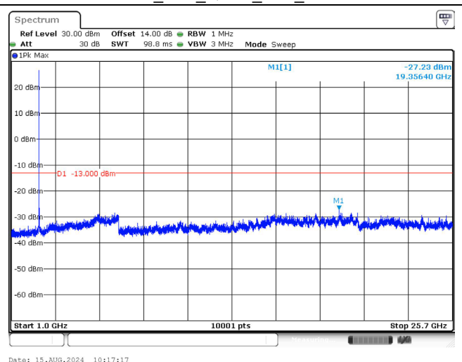
2565.0 MHz_10M_QPSK_1RB_Above 1GHz
