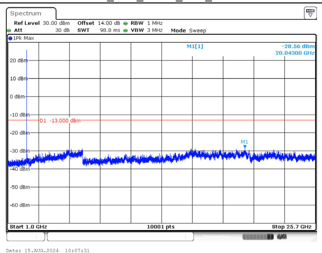
2535.0 MHz_10M_QPSK_1RB_Above 1GHz
