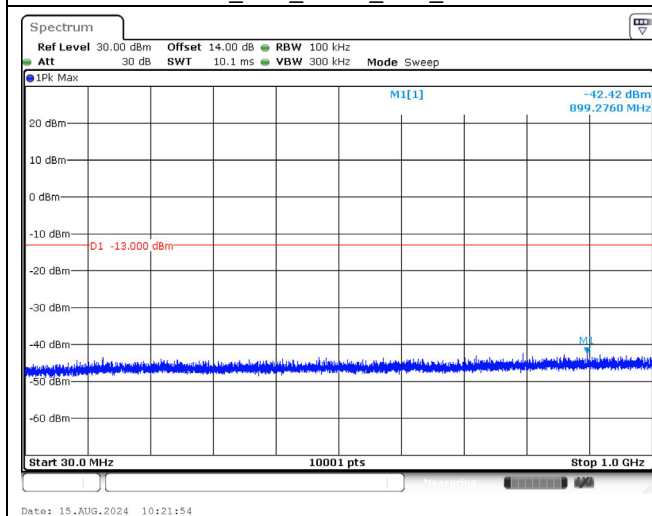
2535.0 MHz_15M_QPSK_1RB_Below 1GHz
