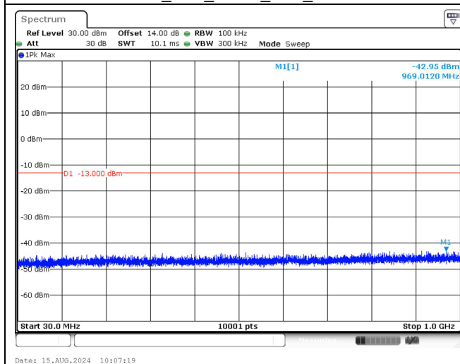
2535.0 MHz_10M_QPSK_1RB_Below 1GHz
