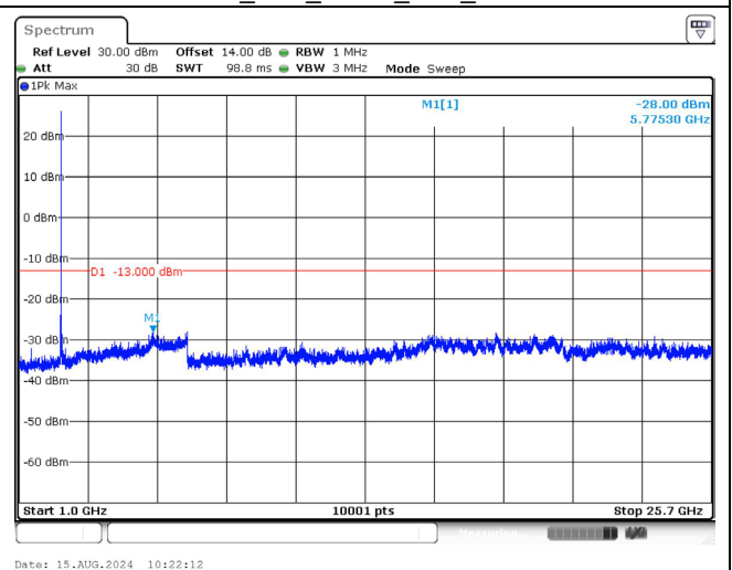
2535.0 MHz_15M_QPSK_1RB_Above 1GHz
