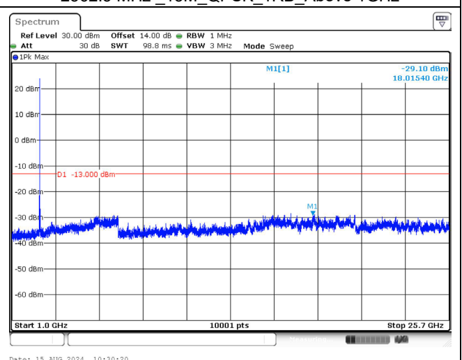
2562.5 MHz_15M_QPSK_1RB_Above 1GHz
