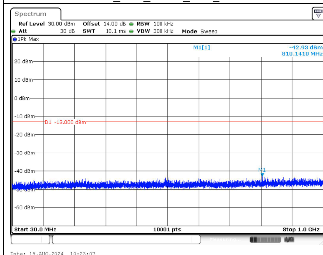
2562.5 MHz_15M_QPSK_1RB_Below 1GHz
