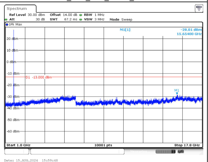
1745.0 MHz_20M_1RB_QPSK_Above 1GHz
