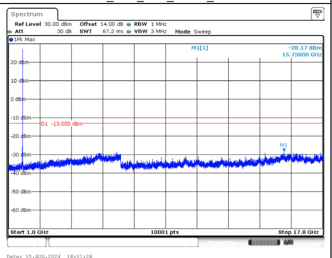
1770.0 MHz_20M_1RB_QPSK_Above 1GHz
