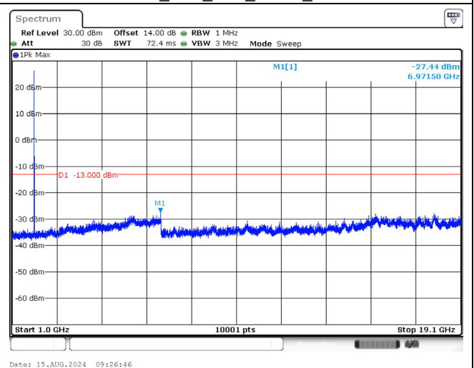
1905.0 MHz_10M_1RB_QPSK_Above 1GHz
