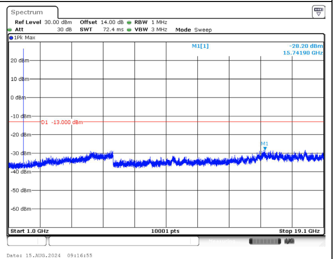
1880.0 MHz_3M_1RB_QPSK_Above 1GHz
