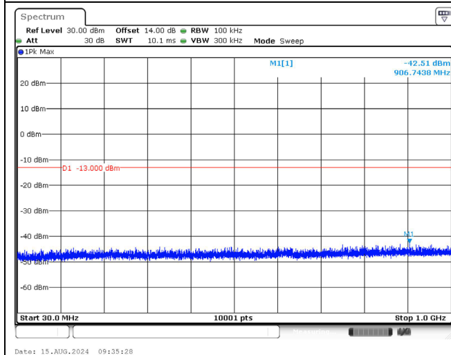
1880.0 MHz_20M_1RB_QPSK_Below 1GHz
