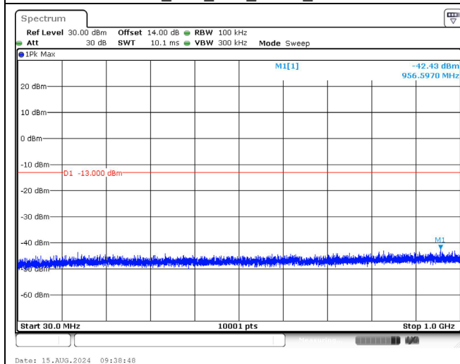
1900.0 MHz_20M_1RB_QPSK_Below 1GHz
