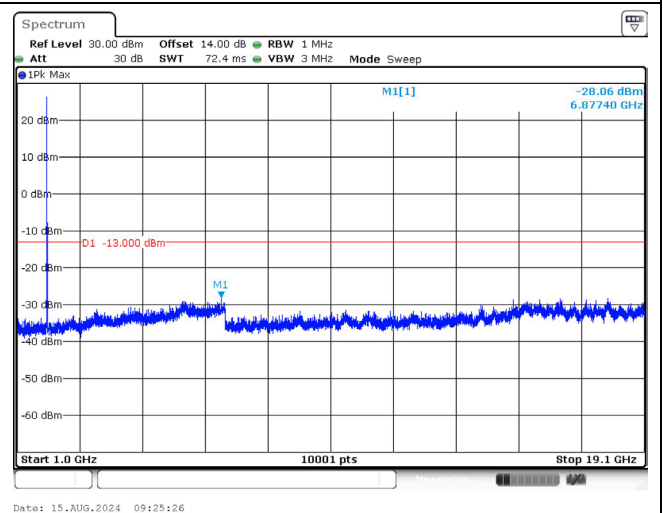
1880.0 MHz_10M_1RB_QPSK_Above 1GHz
