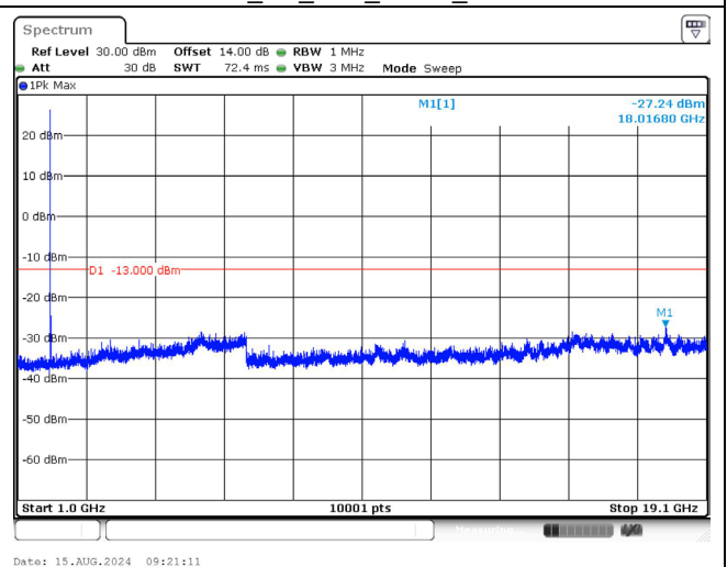
1880.0 MHz_5M_1RB_QPSK_Above 1GHz
