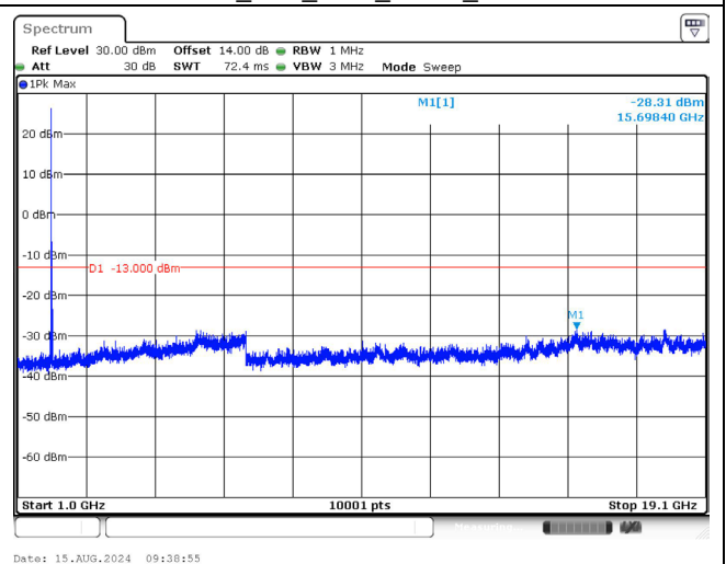
1900.0 MHz_20M_1RB_QPSK_Above 1GHz
