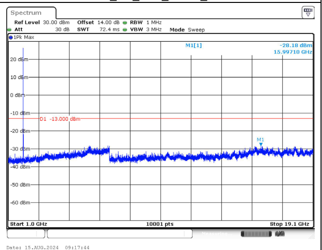
1908.5 MHz_3M_1RB_QPSK_Above 1GHz
