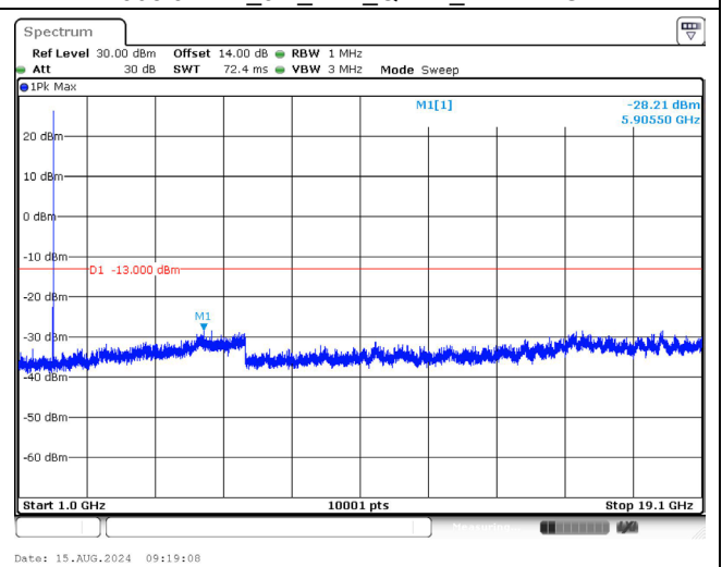
1908.5 MHz_3M_1RB_QPSK_Above 1GHz
