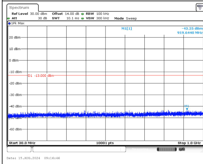
1880.0 MHz_3M_1RB_QPSK_Below 1GHz
