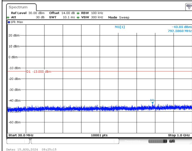
1880.0 MHz_10M_1RB_QPSK_Below 1GHz
