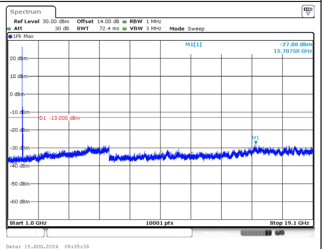
1880.0 MHz_20M_1RB_QPSK_Above 1GHz
