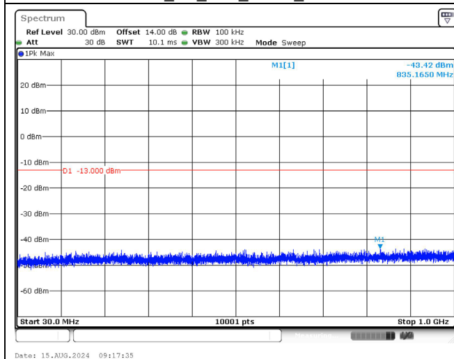
1908.5 MHz_3M_1RB_QPSK_Below 1GHz
