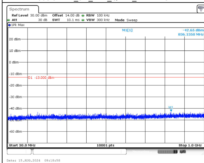
1908.5 MHz_3M_1RB_QPSK_Below 1GHz
