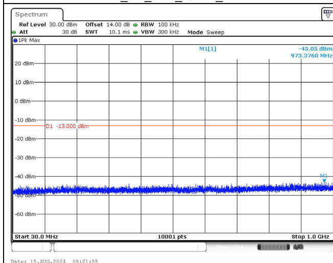
1907.5 MHz_5M_1RB_QPSK_Below 1GHz
