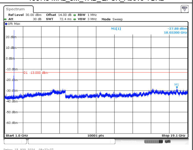
1907.5 MHz_5M_1RB_QPSK_Above 1GHz
