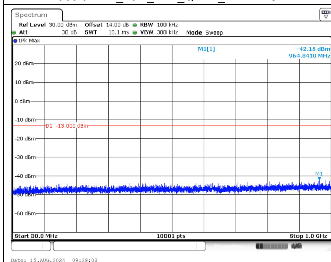
1905.0 MHz_10M_1RB_QPSK_Below 1GHz
