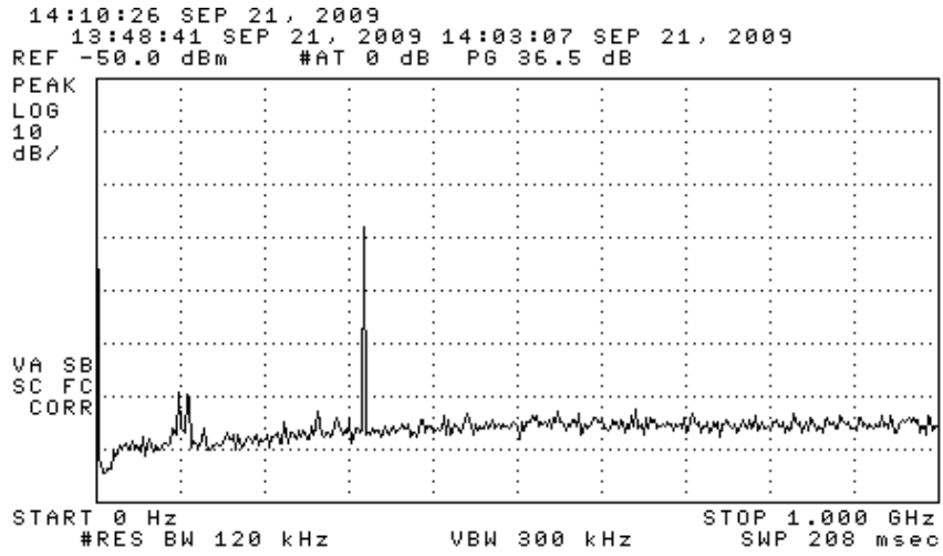
Figure 6.1. Emissions measured at 3 meters in chamber, 0-1000 MHz. (314.9 MHz injected signal is visible)
