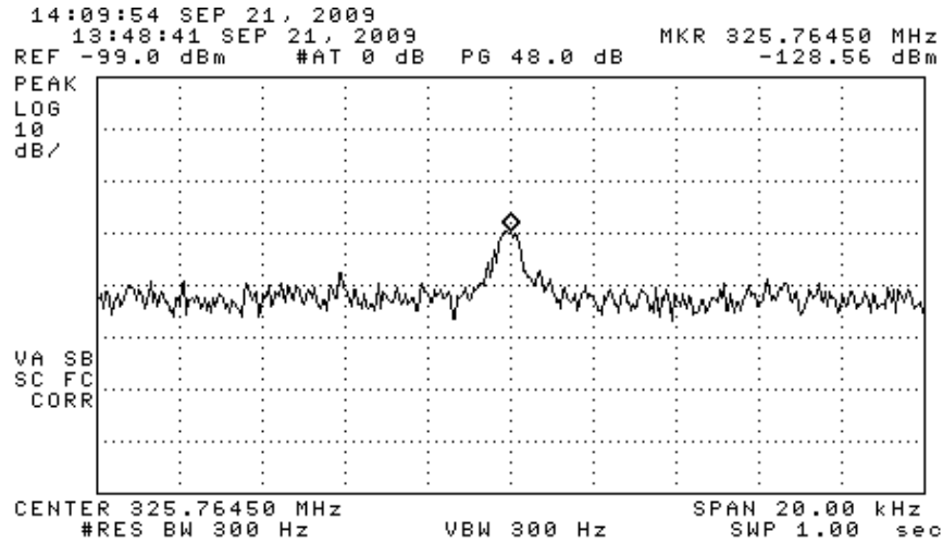
Figure 6.3. Relative receiver emission(s). (No signal could be detected at LO or 2 x LO stated by manufacturer.)
