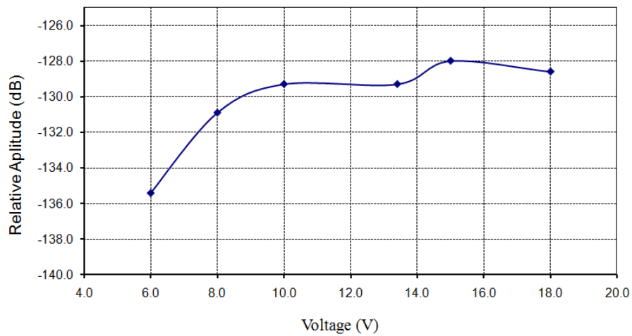
Figure 6.4. Relative 325.7 MHz emission vs. supply voltage.
