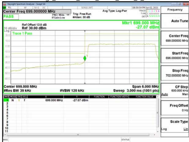
Band Edge_Band12_3MHz_QPSK_RB15_0_CH23025
