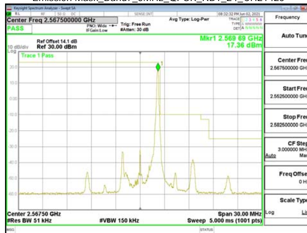
Emission Mask_Band7_5MHz_QPSK_RB1_24_CH21425
