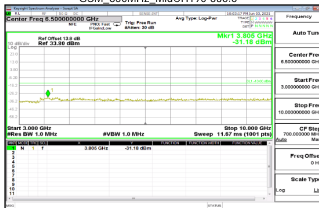
GSM_850MHz_HighCH251-848.8
