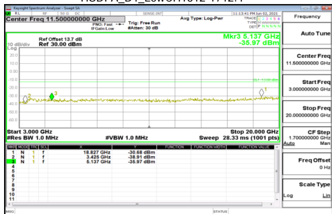
HSDPA_B4_LowCH1312-1712.4
