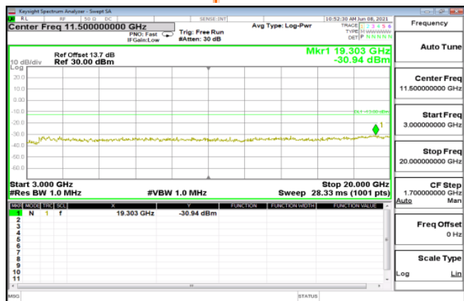
WCDMA_B2_LowCH9262-1852.4
