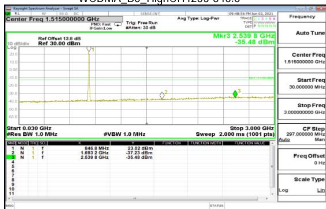
WCDMA_B5_HighCH4233-846.6
