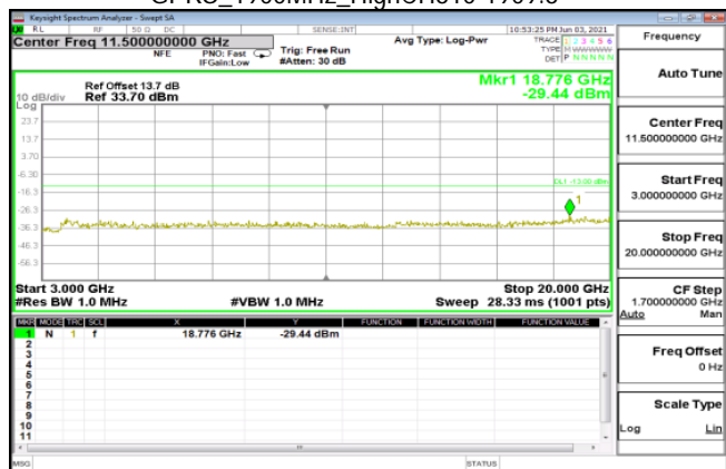
GPRES_1900MHz_HighCH810-1909.8
