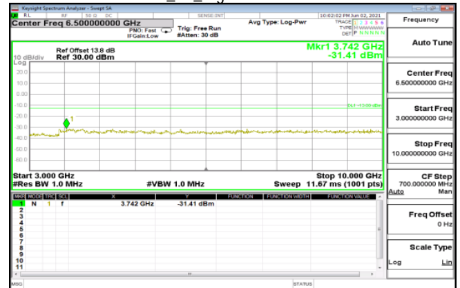
HSUPA_B5_LowCH4132-826.4
