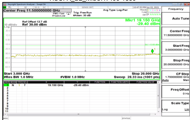
HSUPA_B2_MidCH9400-1880
