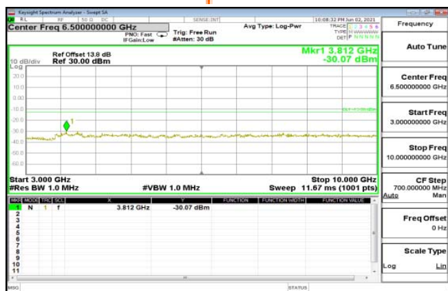
HSUPA_B5_HighCH4233-846.6
