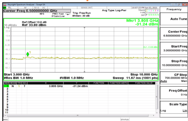
GPRS_850MHz_LowCH128-824.2
