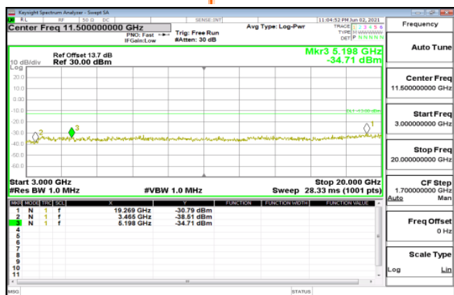
WCDMA_B4_HighCH1513-1752.6
