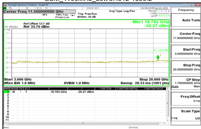
GSM_1900MHz_LowCH512-1850.2
