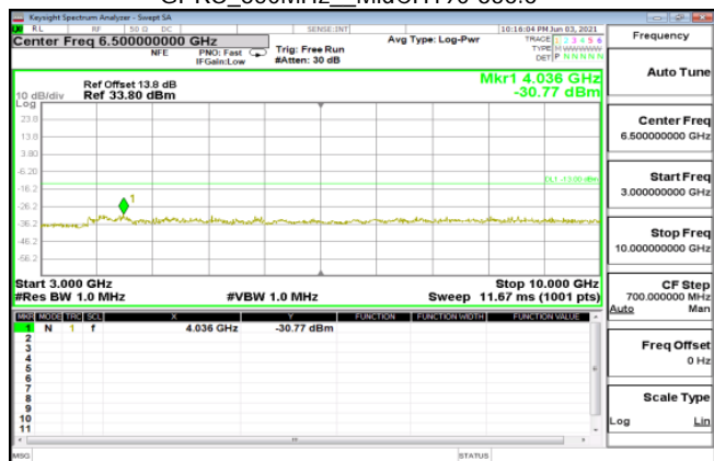
GPRS_850MHz_MidCH190-836.6
