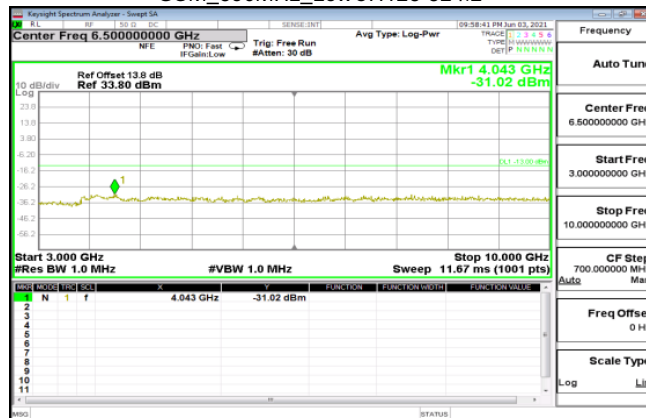
GSM_850MHz_MidCH190-836.6
