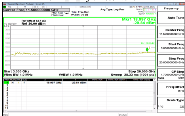
HSUPA_B2_LowCH9262-1852.4
