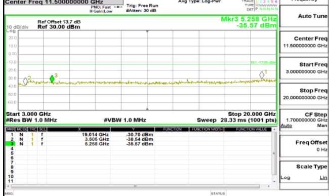
HSUPA_B4_HighCH1513-1752.6
