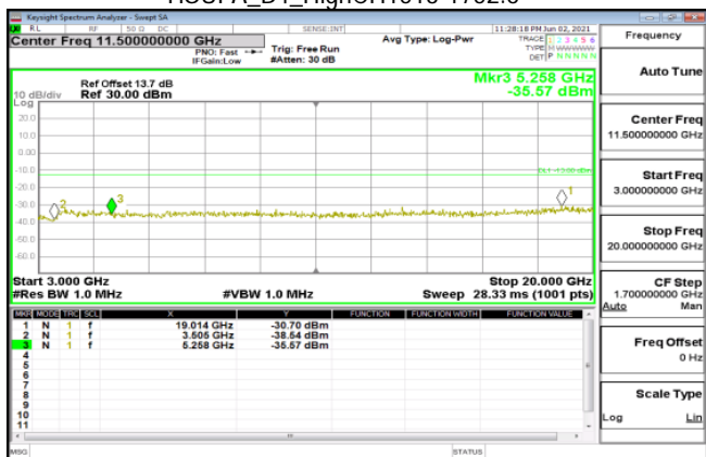
HSUPA_B4_HighCH1513-1752.6
