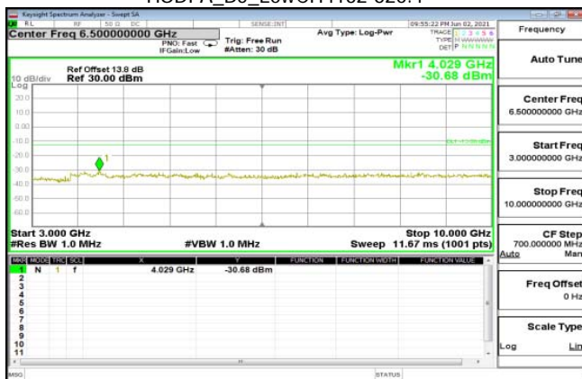
HSDPA_B5_MidCH4183-836.6
