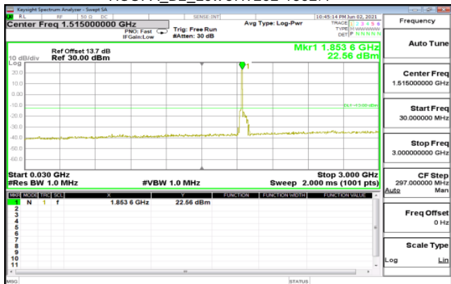
HSUPA_B2_MidCH9400-1880
