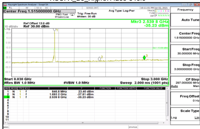
HSUPA_B5_HighCH4233-846.6
