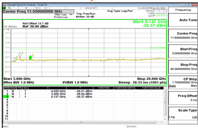
HSUPA_B4_MidCH1413-1732.6
