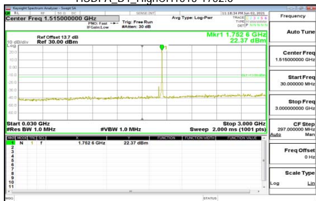
HSDPA_B4_HighCH1513-1752.6
