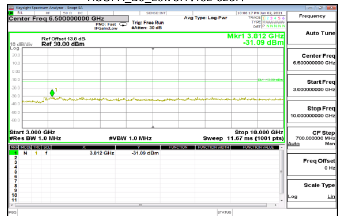
HSUPA_B5_MidCH4183-836.6
