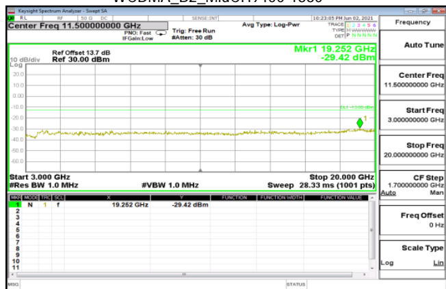
WCDMA_B2_MidCH9400-1880
