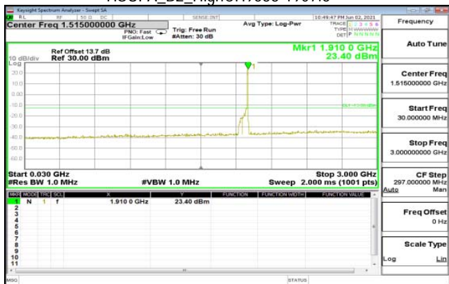
HSUPA_B2_HighCH9538-1907.6
