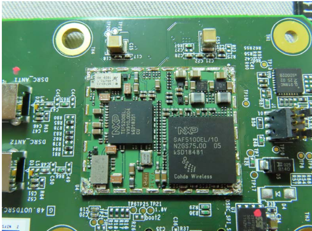
Internal View of EUT – 16
