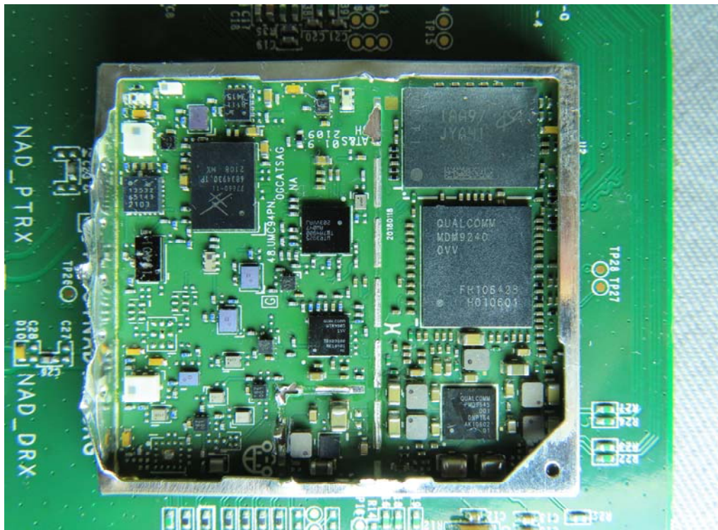
Internal View of EUT – 18
