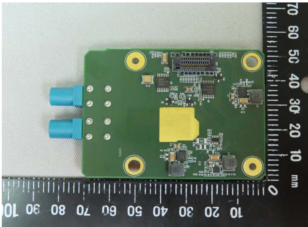
Internal View of EUT – 14
