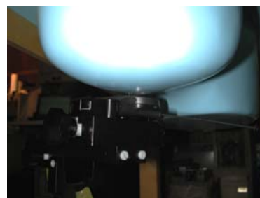
Figure 21. Left Head SAR Test Setup -- Ear / Tilt Position --
