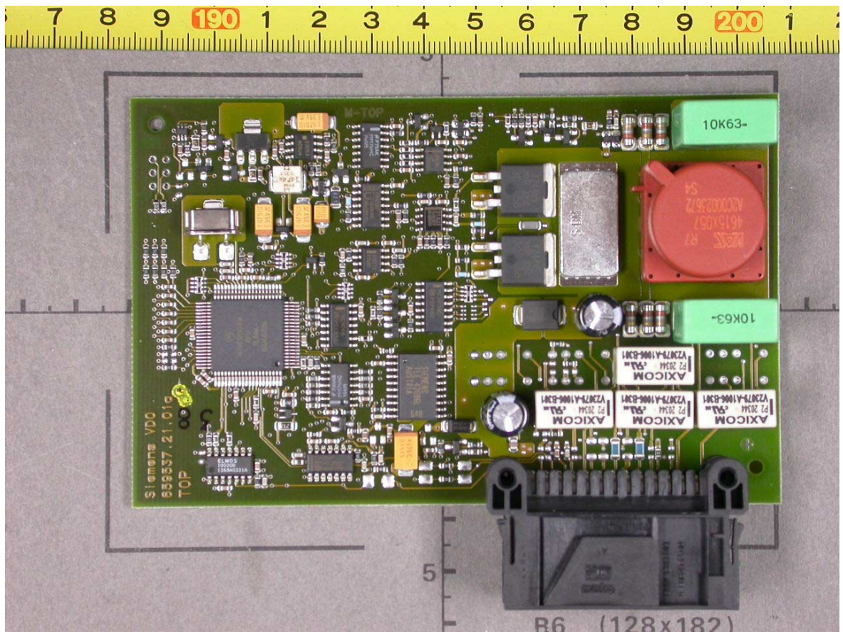
Top view of printed board (Control-unit)
