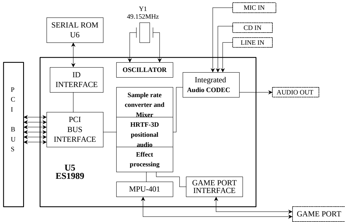
A571-T70 BLOCK DIAGRAM
