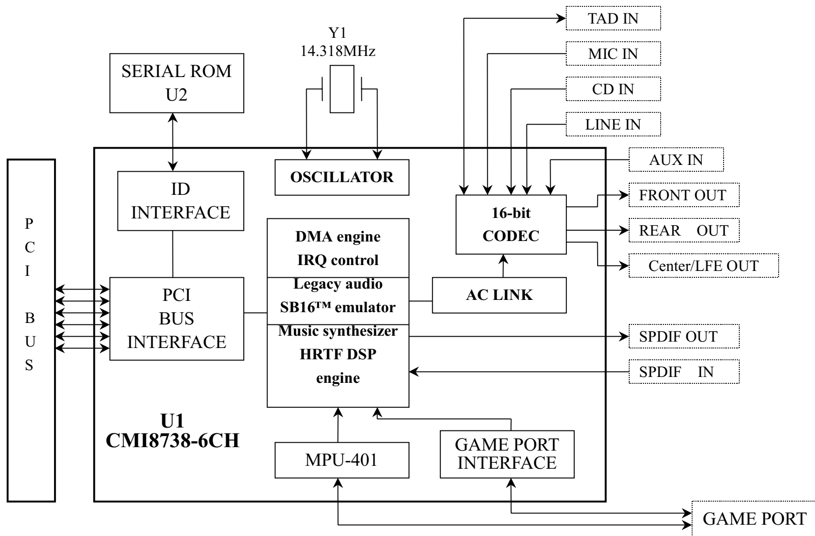
A521-T90 BLOCK DIAGRAM
