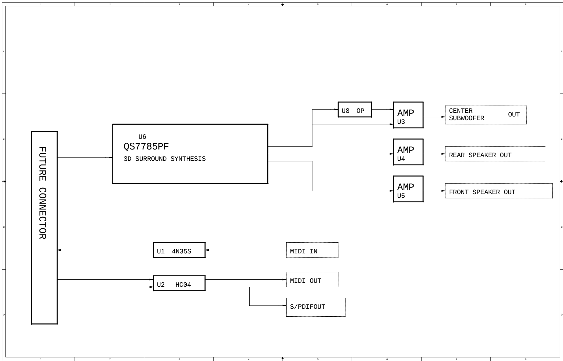
A461-L00 BLOCK DIAGRAM
