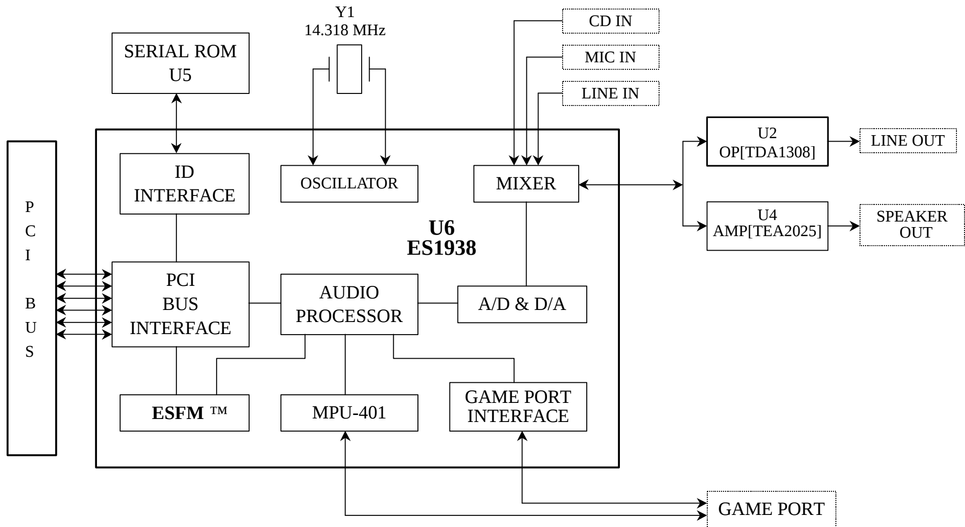
A331-L70 BLOCK DIAGRAM
