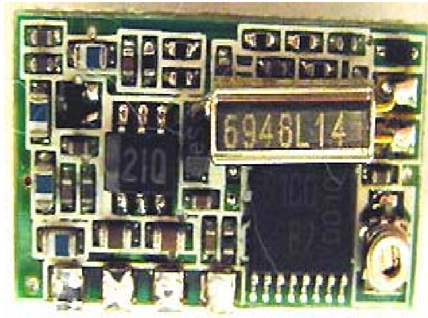
Transmitter PCB Rear View
