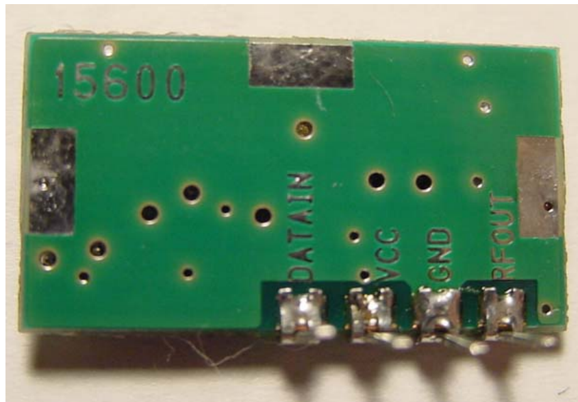
Transmitter PCB Rear View
