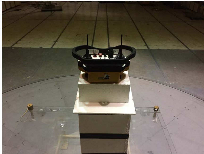
Radiated Emissions C63.10, Back
