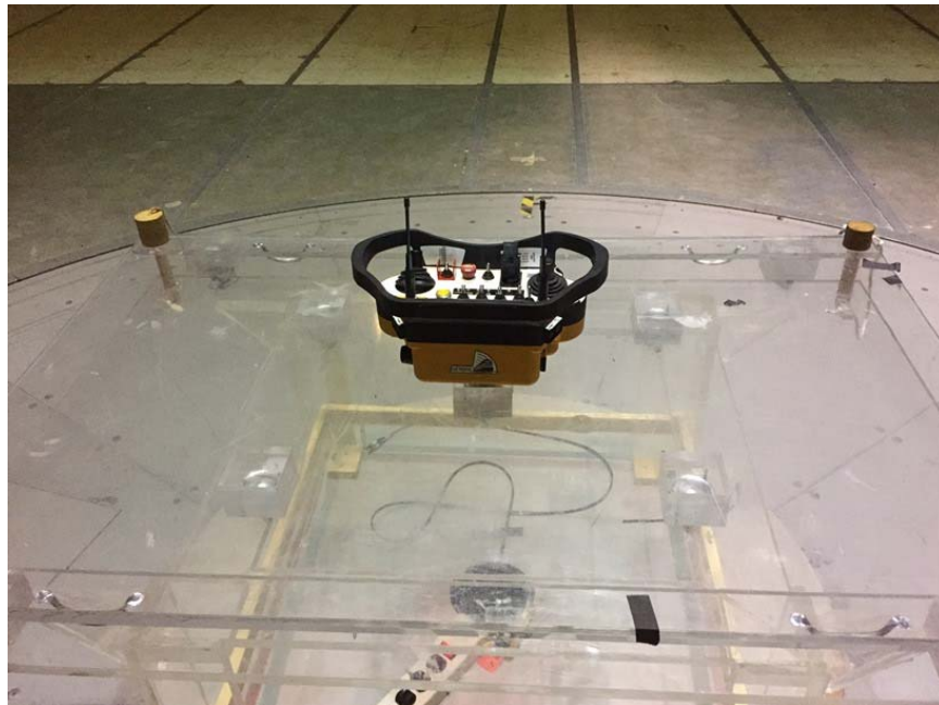
Radiated Emissions to 1 GHz, Back
