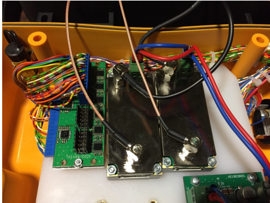
Amplifiers
