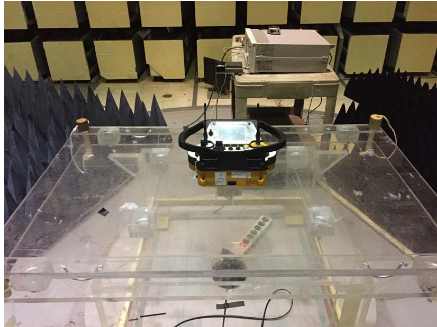
Radiated Emissions to 25 GHz, Front
