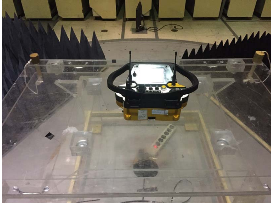
Radiated Emissions to 1 GHz, Front
