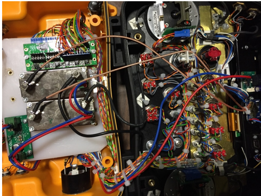
EUT Setup, Overall
