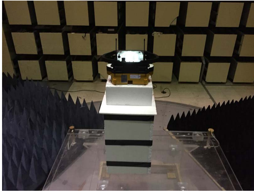
Radiated Emissions C63.10, Front
