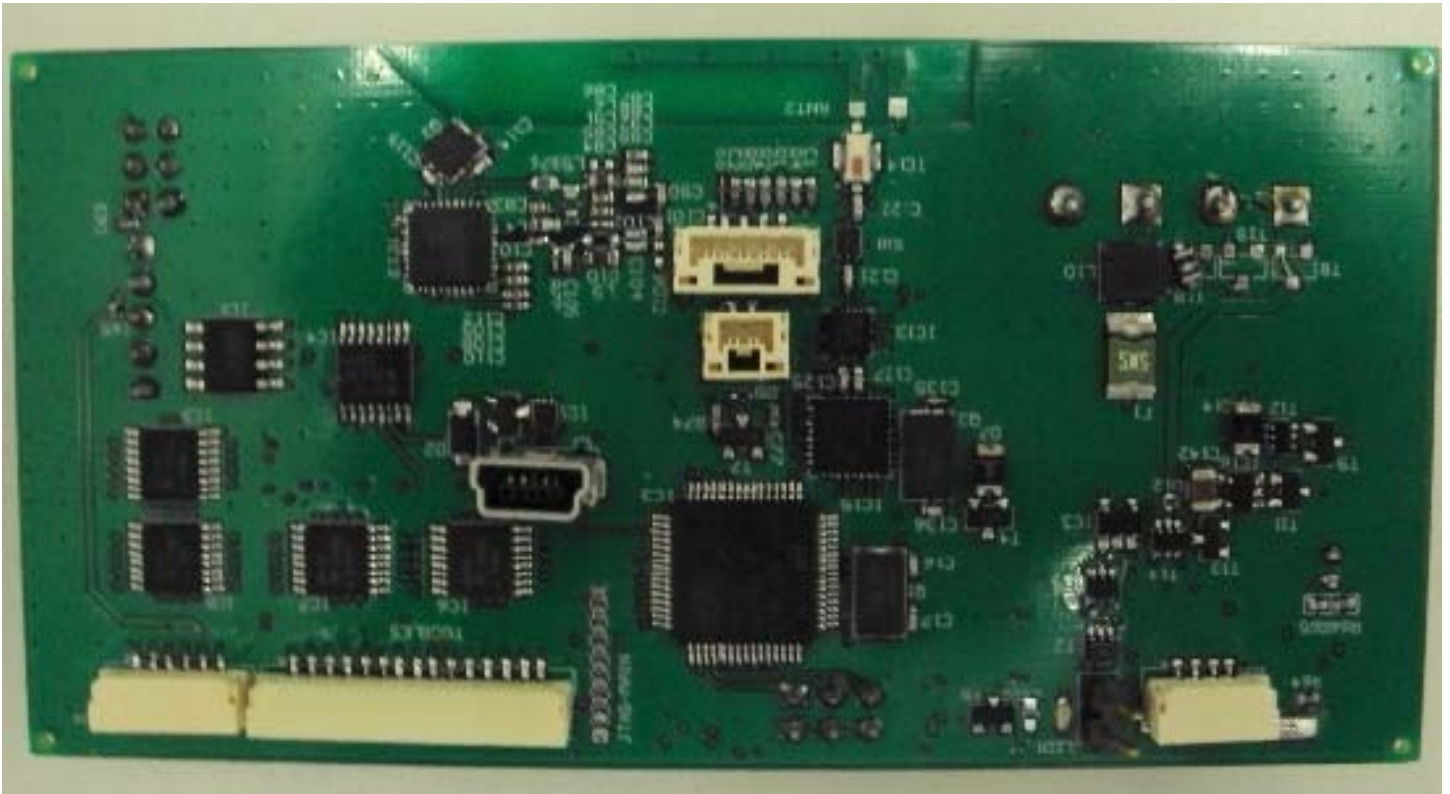
BOTTOM VIEW
