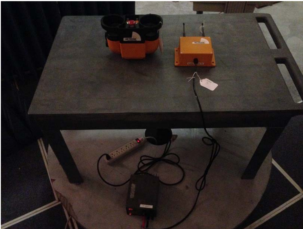
Radiated Emissions 18-25 GHz Back
