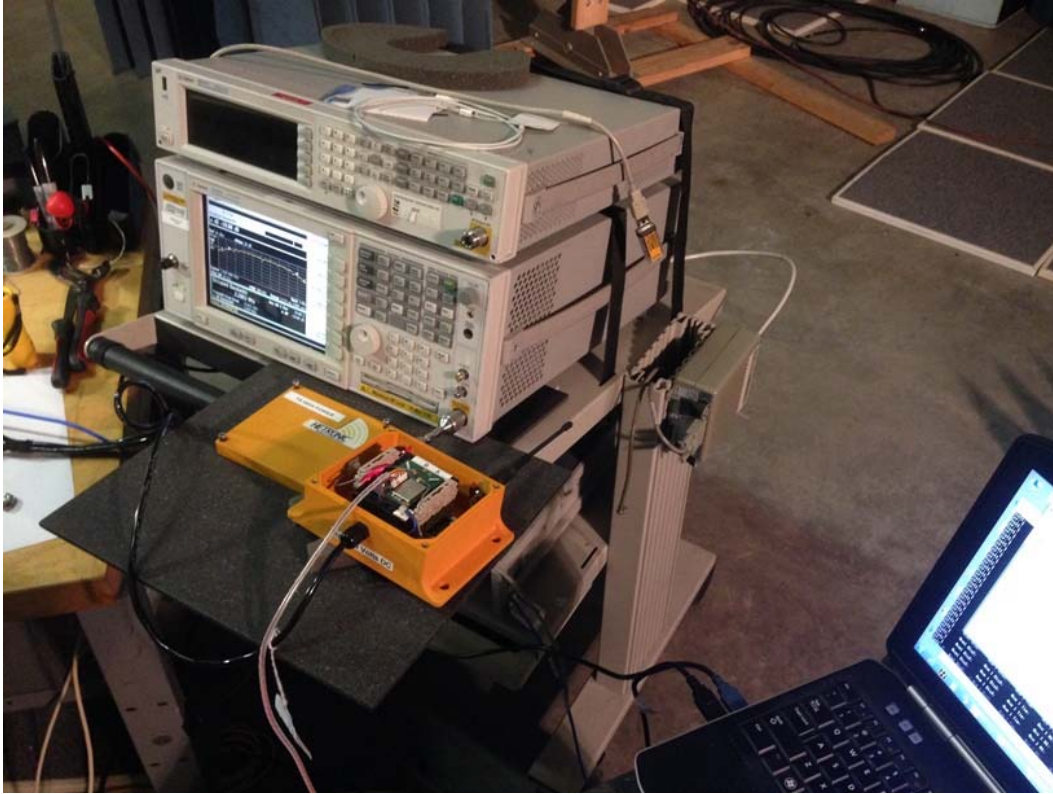
Antenna Port Conducted, Power, PSD, Bandwidth
