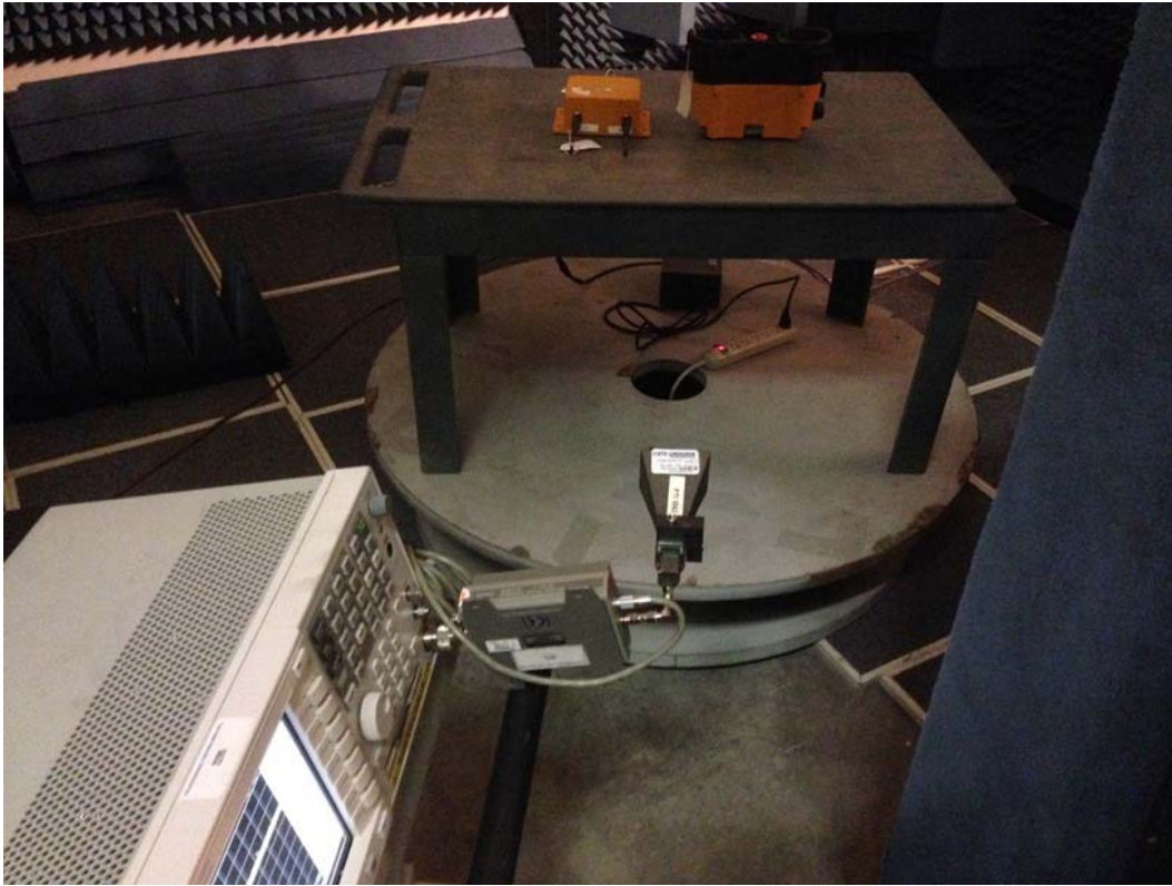
Radiated Emissions 18-25 GHz Front
