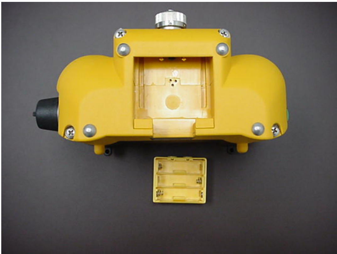
Rear View Battery Compartment and Battery Holder
