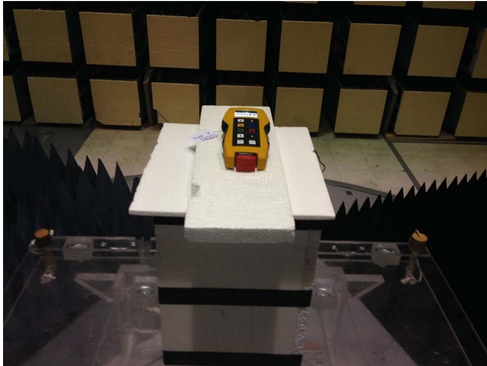
Radiated Emissions to 18 GHz; Power, Spurious; Front
