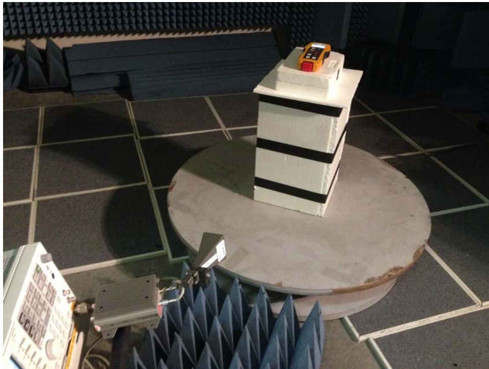
Radiated Emissions 18-25 GHz; Spurious
